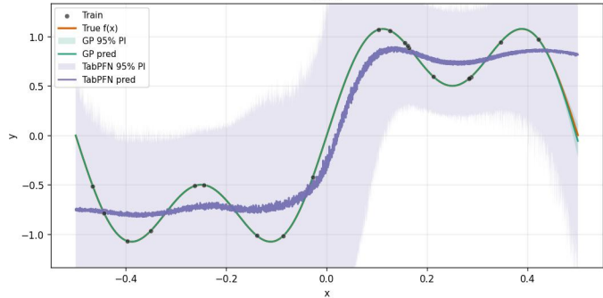
A22_smooth_multisine_1Dx_20Dn_[-0.5,0.5]_16inits_noiseTest0.0_noiseTrain0.0_x10 run 1
