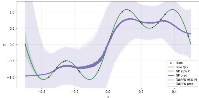
A22_smooth_multisine_1Dx_20Dn_ [-0.5, 0.5] _16inits_noiseTest0.0_noiseTrain0.0_x10 run 8
