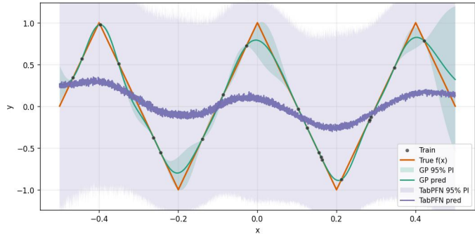
A22_triangle_wave_1Dx_20Dn_ [-0.5, 0.5] _16inits_noiseTest0.0_noiseTrain0.0_x10 run 1
