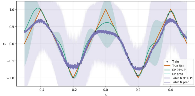
A22_triangle_wave_1Dx_20Dn_ [-0.5, 0.5] _16inits_noiseTest0.0_noiseTrain0.0_x10 run 7
