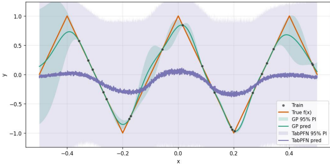
A22_triangle_wave_1Dx_20Dn_ [-0.5, 0.5] _16inits_noiseTest0.0_noiseTrain0.0_x10 run 8
