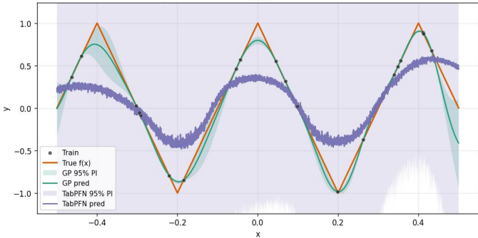
A22_triangle_wave_1Dx_20Dn_ [-0.5, 0.5] _16inits_noiseTest0.0_noiseTrain0.0_x10 run 3
