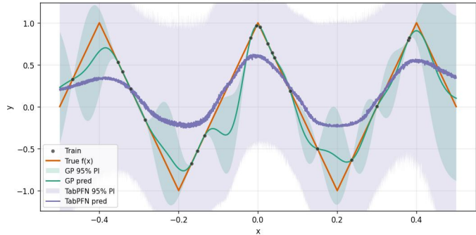
A22_triangle_wave_1Dx_20Dn_ [-0.5, 0.5] _16inits_noiseTest0.0_noiseTrain0.0_x10 run 10
