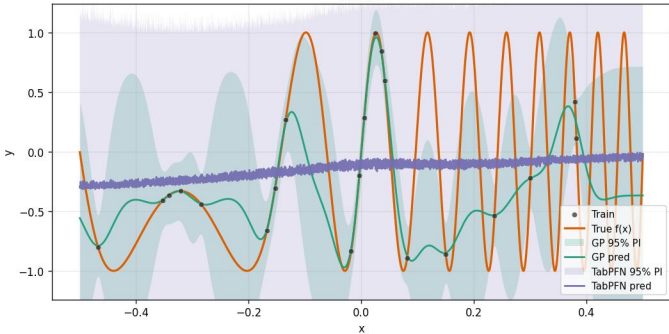
A22_chirp_1Dx_20Dn_ [-0.5, 0.5] _16inits_noiseTest0.0_noiseTrain0.0_x10 run 10
