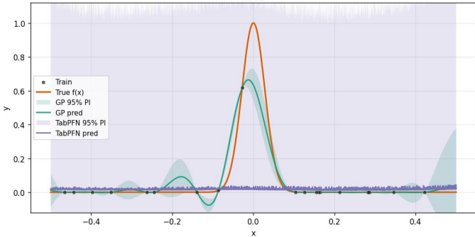
A22_localized_bump_1Dx_20Dn_ [-0.5, 0.5] _16inits_noiseTest0.0_noiseTrain0.0_x10 run 1
