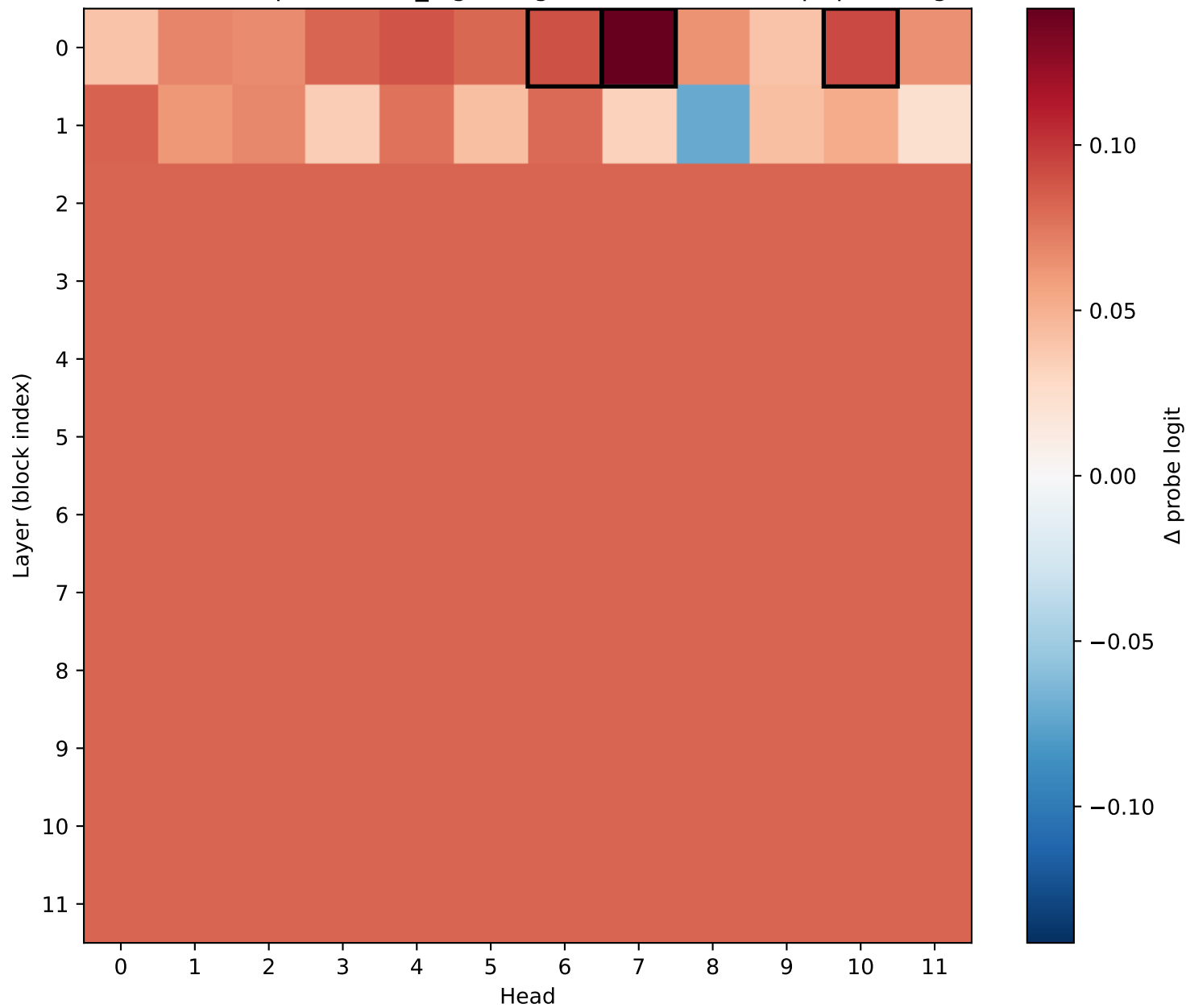
BIOS BERT — per-head \Delta_{\text{logit}} on gender (clean→corrupt patching)
