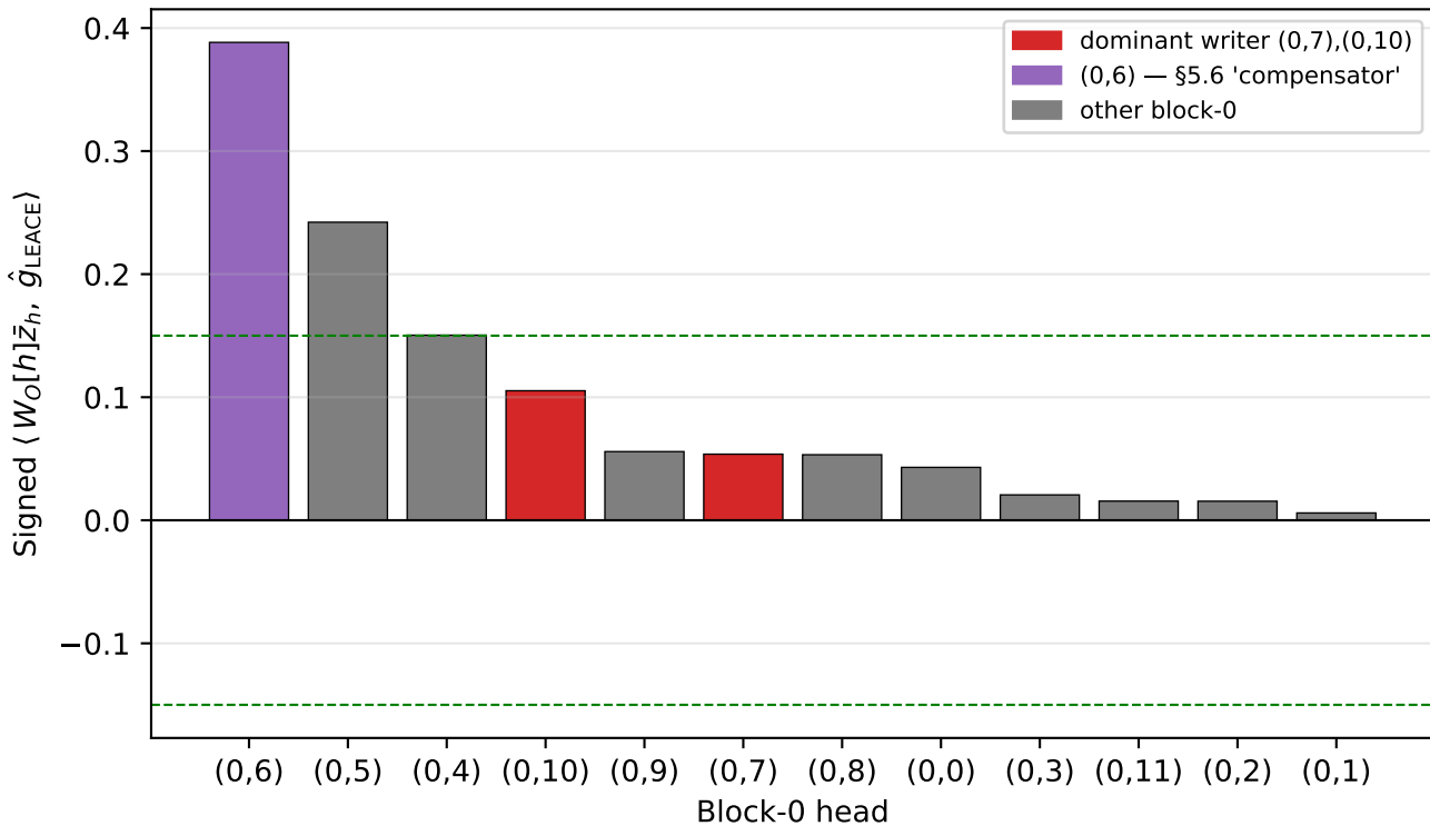
Block-0 head OV writes along the LEACE rank-1 gender direction ALL 12 heads project positively — no directional compensators
