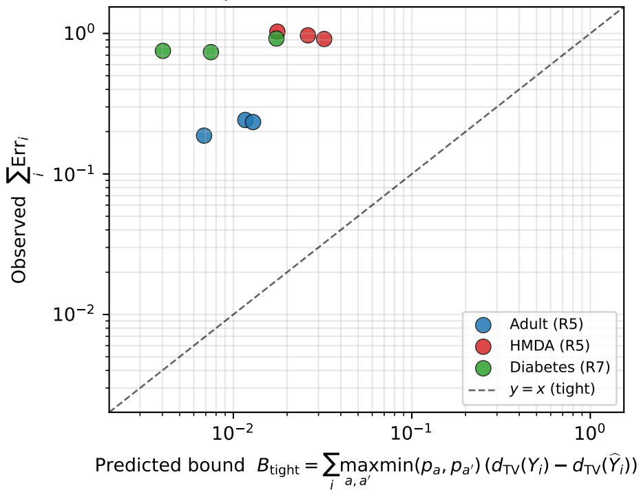
PCRL: observed total error vs. d_{TV} corollary lower bound (per-seed, attribute = race)
