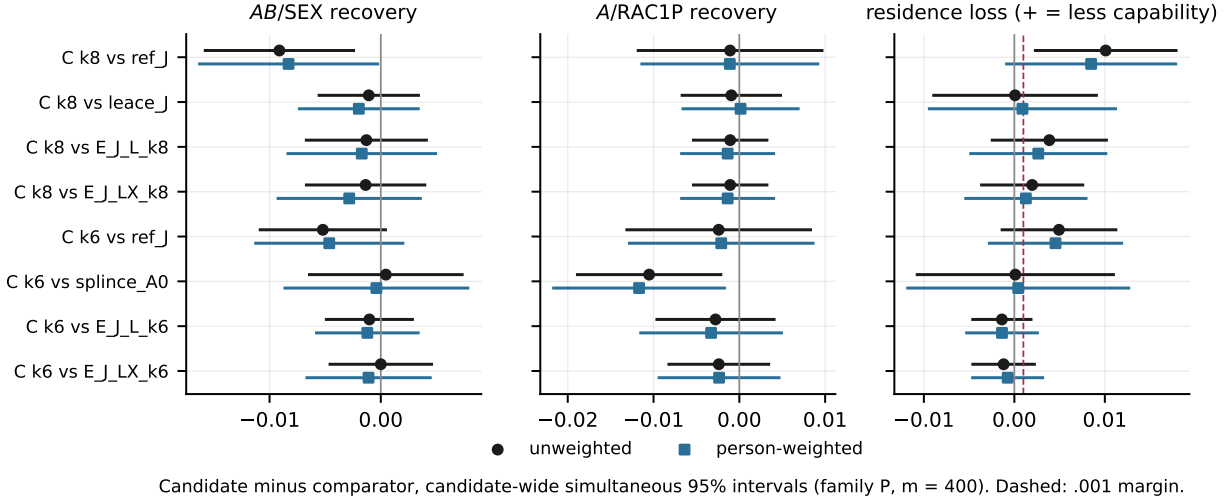
Figure 5: Study 5 panel contrasts, candidate minus comparator, candidate-wide simultaneous 95% intervals in family P ( m = 400 ), both weightings. For recovery, negative is less disclosure; for residence loss, positive is less capability; dashed line: the 0.001 margin. Among the rows drawn, only the J comparison on AB/SEX (both weightings) and SPLINCE on A/RAC1P resolve in the candidate’s favour; neither is accompanied by residence noninferiority. Table form with all endpoints: Appendix I.
