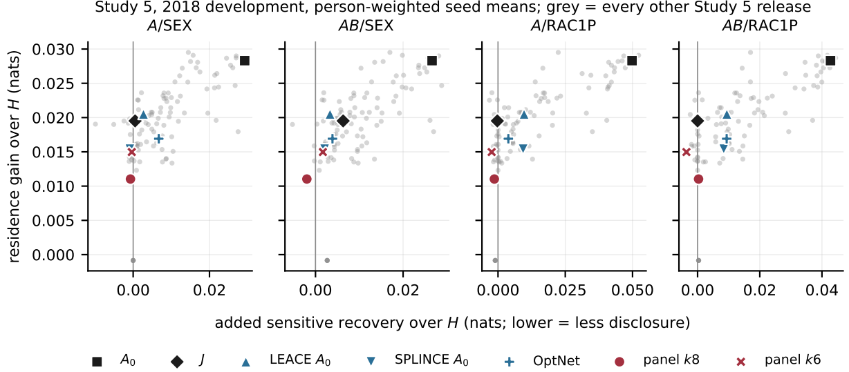
Figure 8: Study 5, 2018, person-weighted counterpart of Figure 4.
