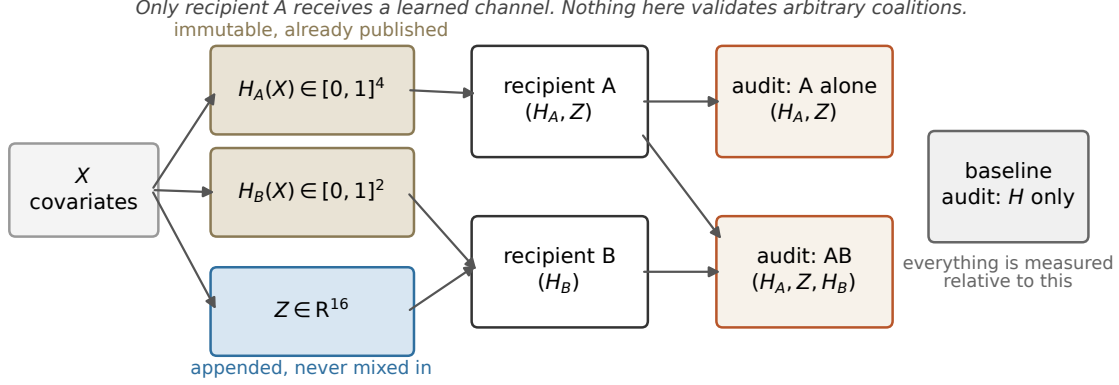
Figure 1: The release graph. H_A and H_B are already published and never modified; Z is appended to A ’s wire alone. Three audit views are scored: A alone, the coalition AB , and the H -only baseline every increment is measured against. A schematic, not a result.
