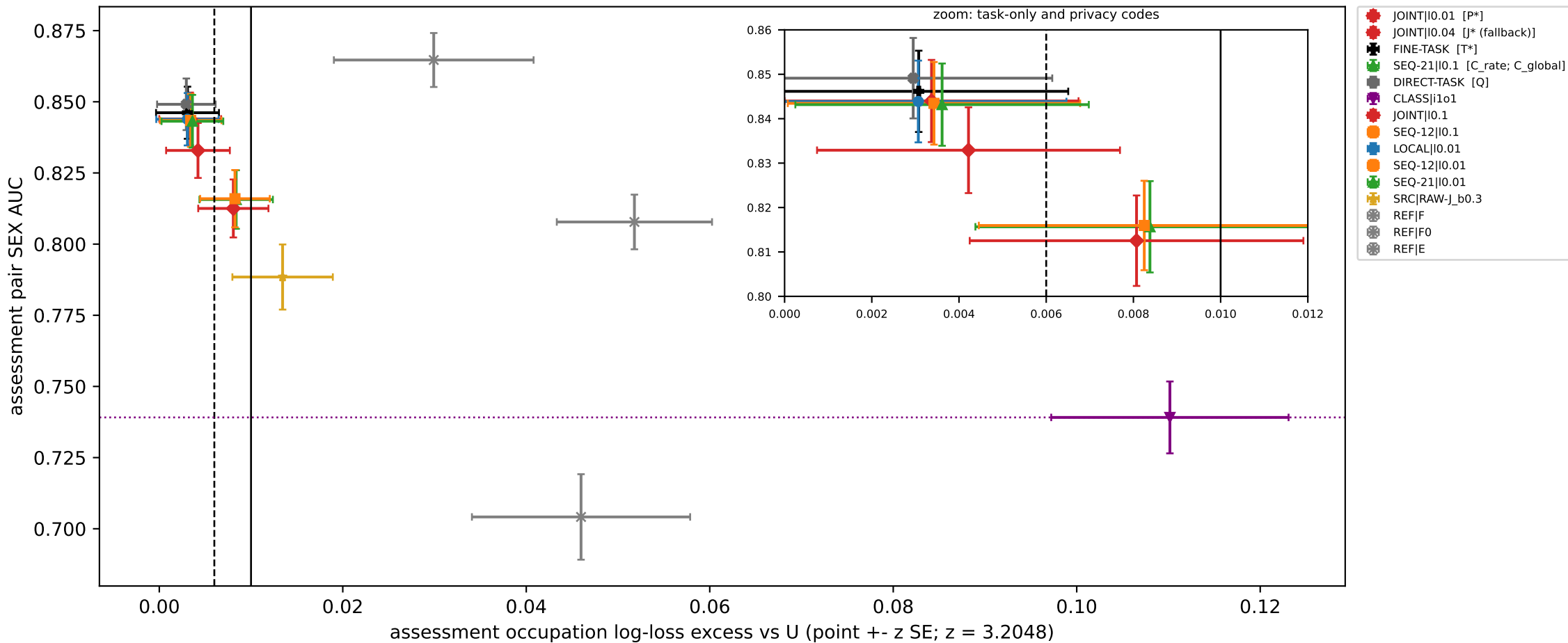
Figure 2: locked scored list (dashed: 0.006 inner headroom; solid: 0.01 allowance; dotted: CLASS-ONLY)
