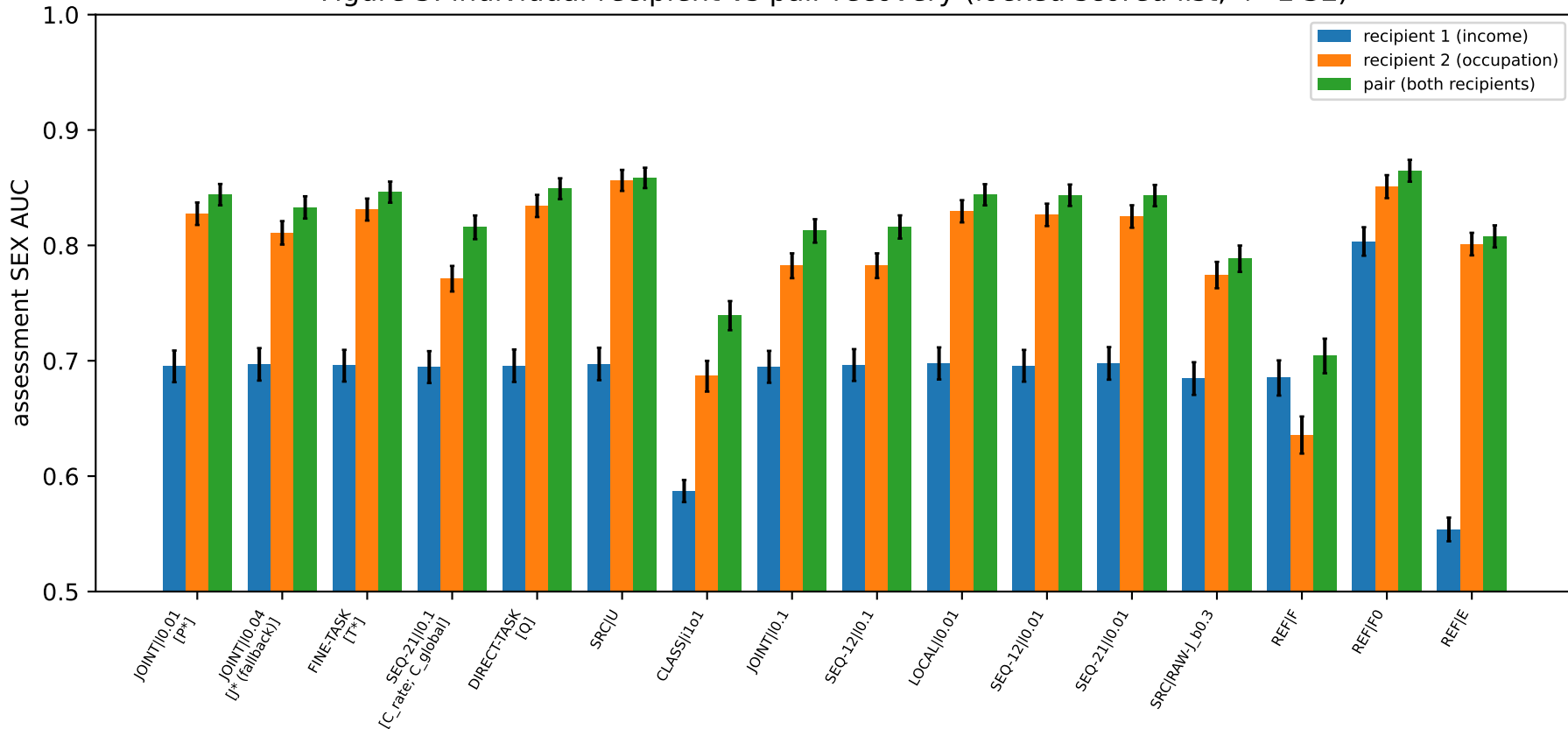
Figure 3: individual-recipient vs pair recovery (locked scored list; \pm z SE)
