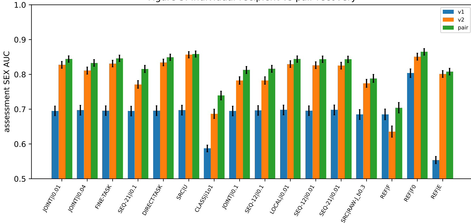
Figure 3: individual-recipient vs pair recovery
