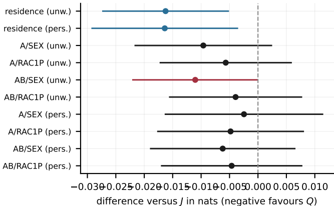
Selected release Q against J (development; simultaneous adjusted bounds, m = 706 )
