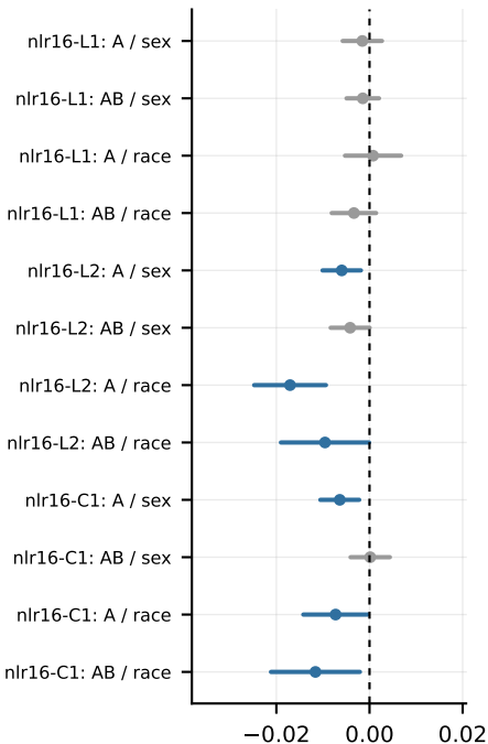
Nonlinear penalty, r = 16
