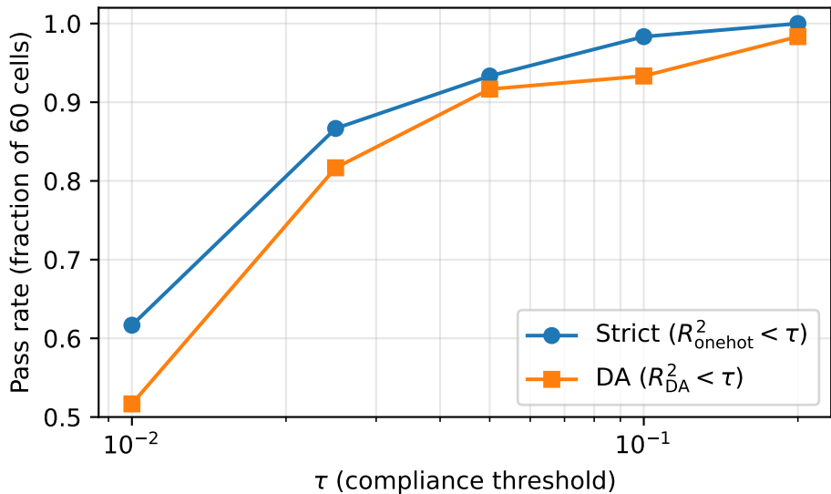
Pass-rate sensitivity to \tau (60 cells, 3 datasets \times 3 seeds)
