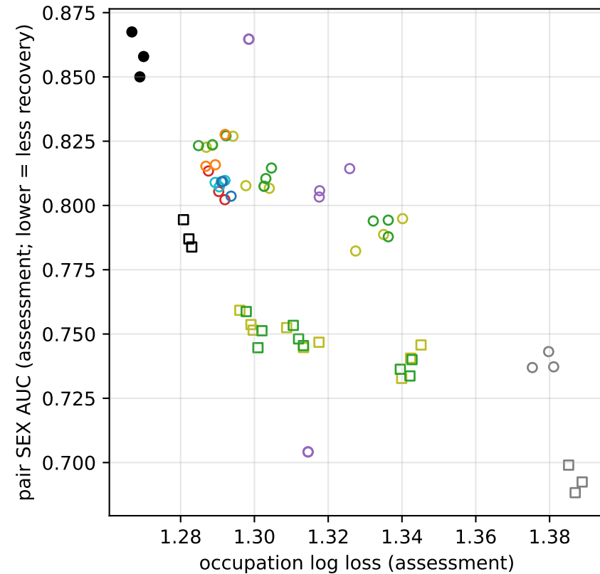
Pair recovery vs task log loss and accuracy; filled = inner task-eligible; squares = RAW-J teacher
