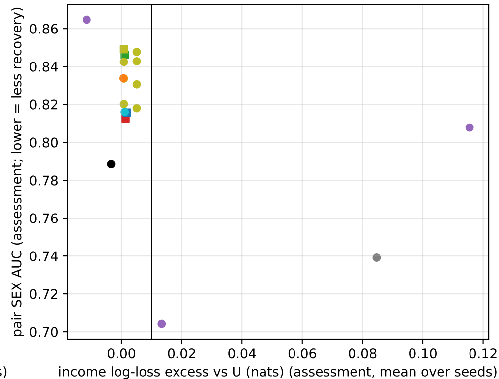
Recovery vs confidence and accuracy (squares = selected roles; line = 0.01-nat allowance)
