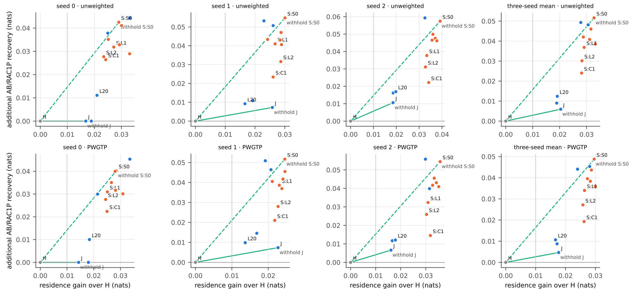
Mode A (kernel_expanded_catchup, budget 360): residence gain vs additional AB/RAC1P recovery. Orange spectral, blue neural, gray H, green withholding (p=0.1). Dotted line: .01 reference.
