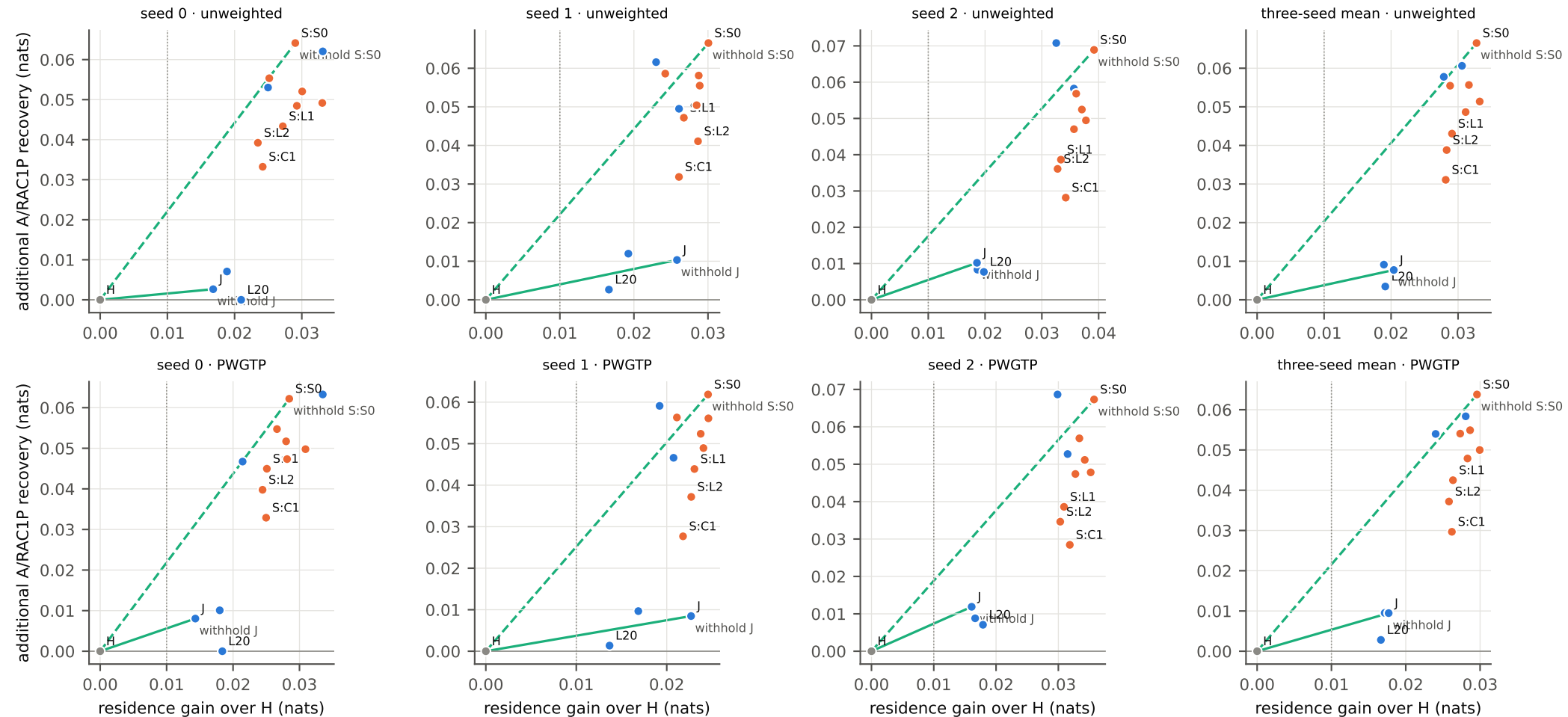
Mode A (kernel_expanded_catchup, budget 360): residence gain vs additional A/RAC1P recovery. Orange spectral, blue neural, gray H, green withholding (p=0.1). Dotted line: .01 reference.
