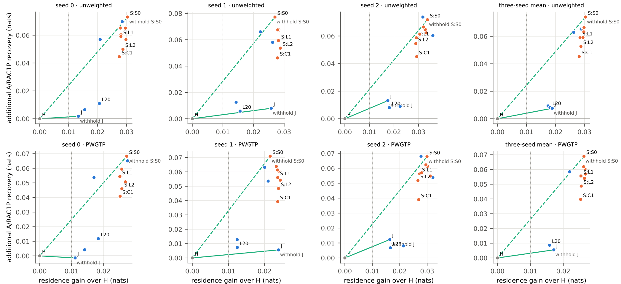
Mode B (transport_all, budget 360): residence gain vs additional A/RAC1P recovery. Orange spectral, blue neural, gray H, green withholding (p=0..1). Dotted line: .01 reference.
