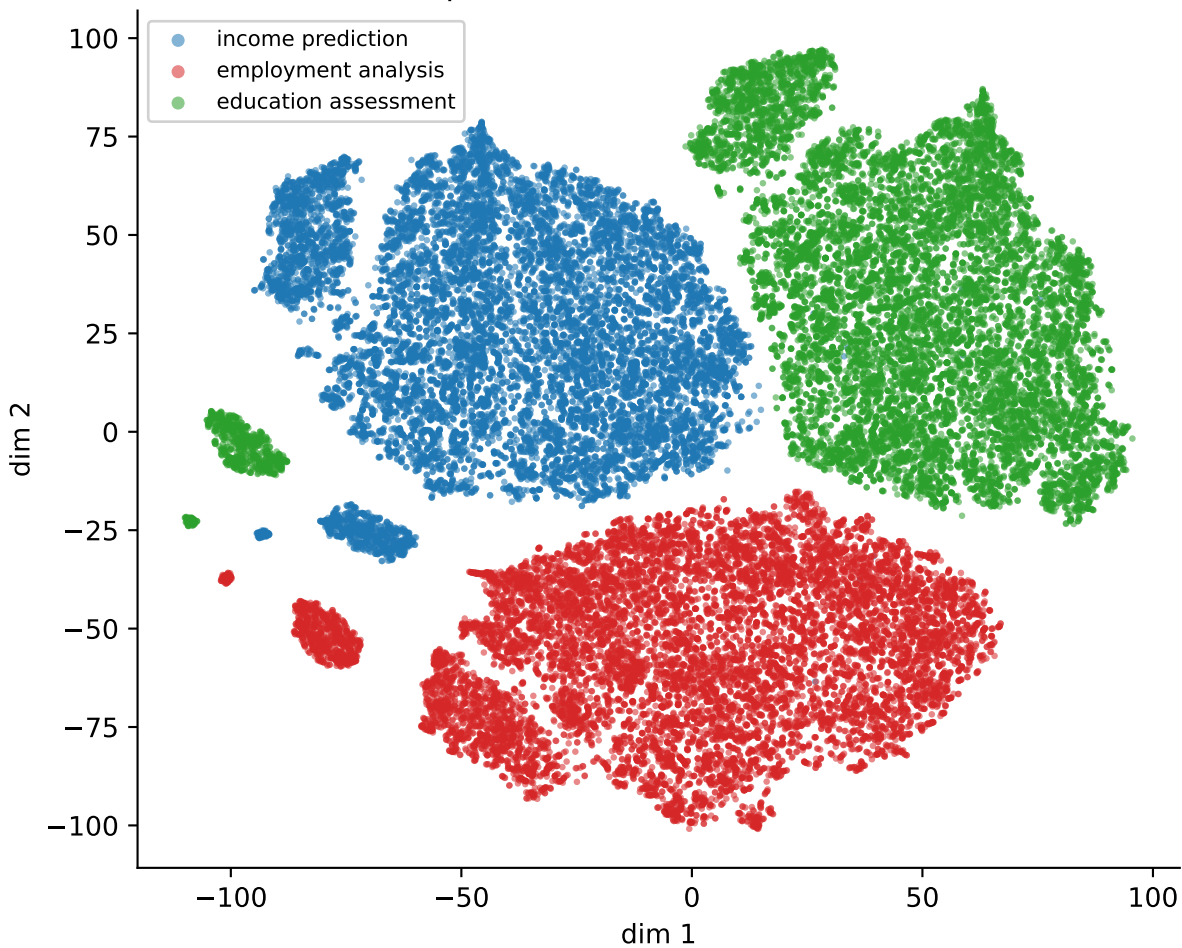
Adult — PCRL representations (t-SNE) (silhouette = 0.413)
