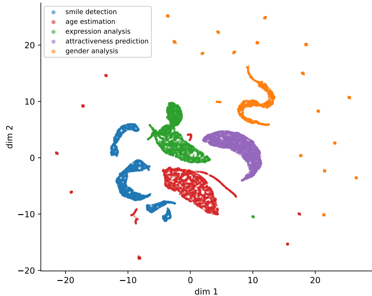
CelebA — PCRL representations (UMAP) (silhouette = 0.293)
