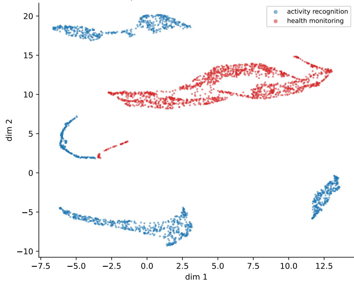
HAR — PCRL representations (UMAP) (silhouette = 0.309)
