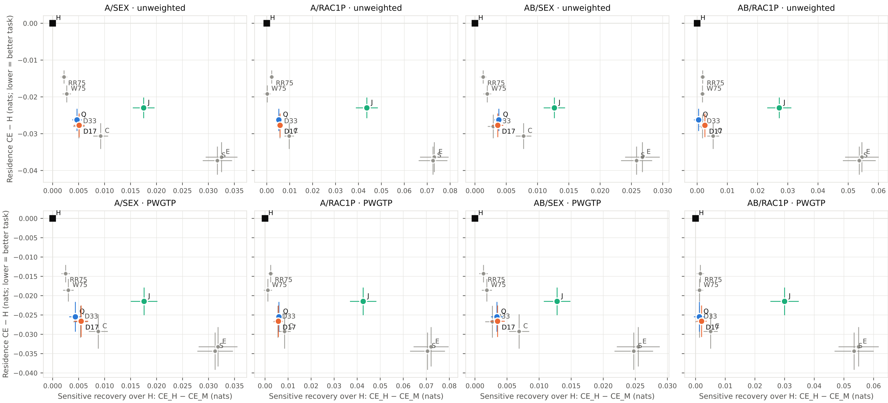
ACS 2016 final pool: task gain versus measured sensitive recovery, per role and weighting mean of three anchors; bars = unadjusted marginal 95% household-bootstrap intervals (descriptive)
