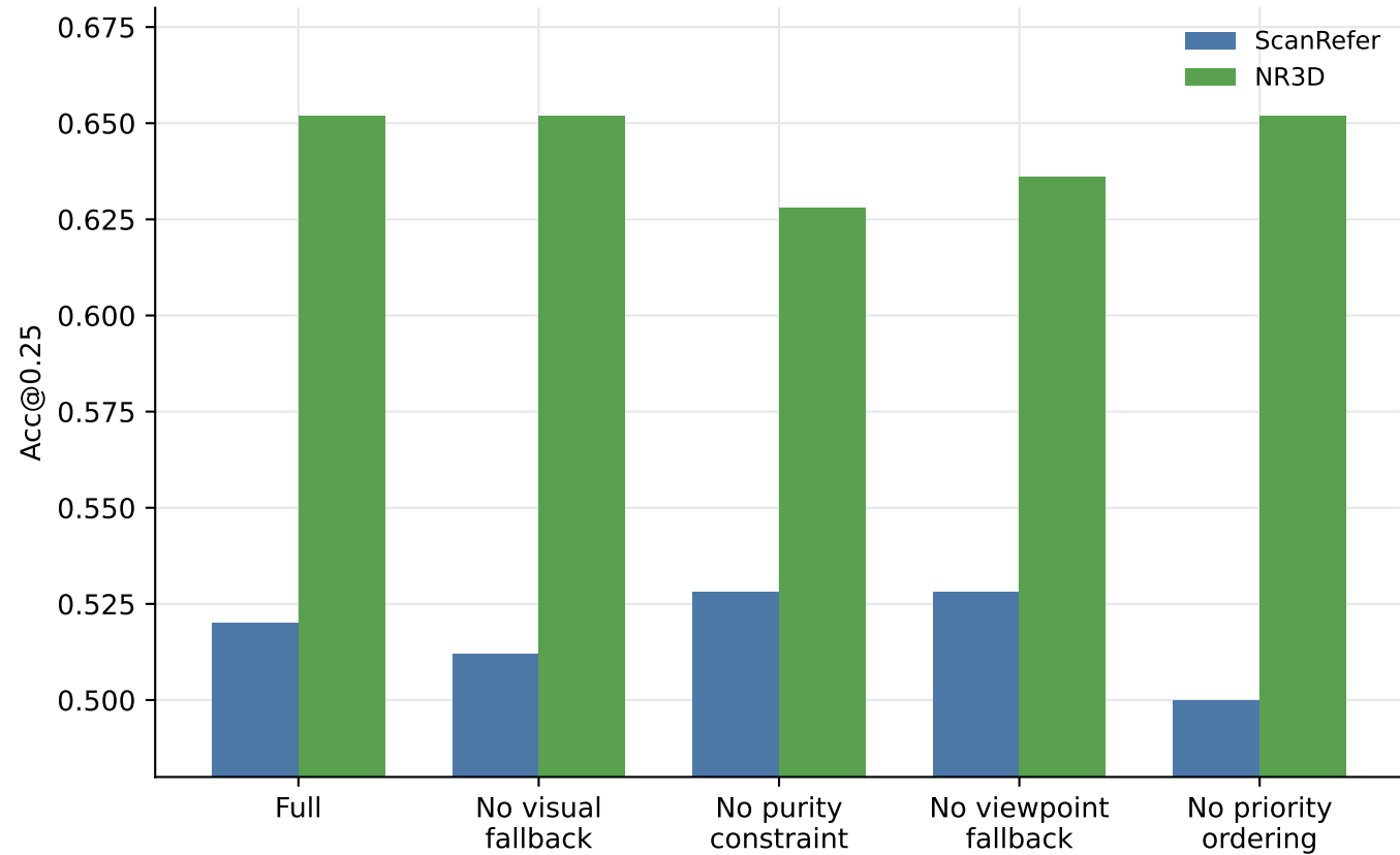
Router Component Ablation
