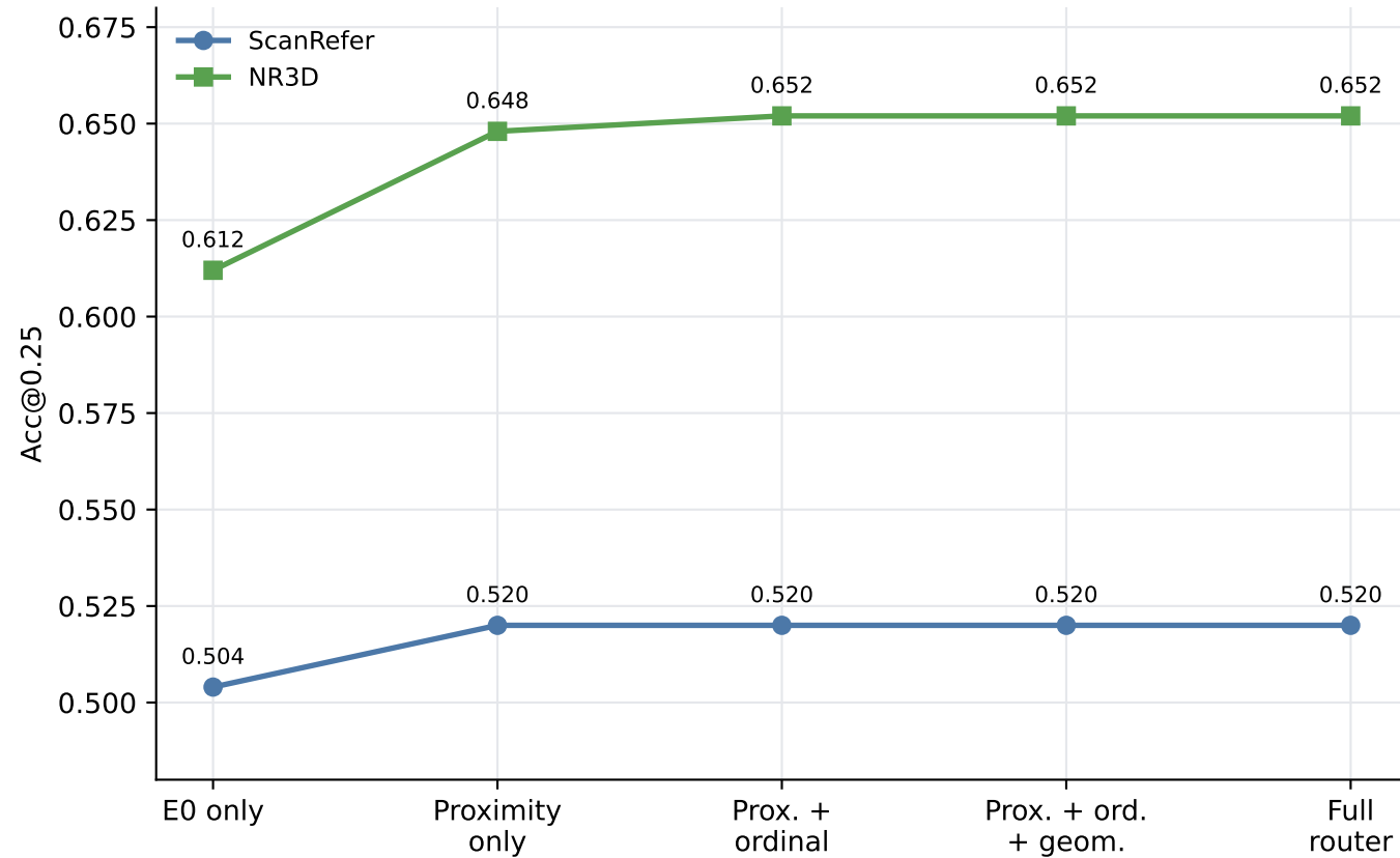
Cumulative Policy Ablation
