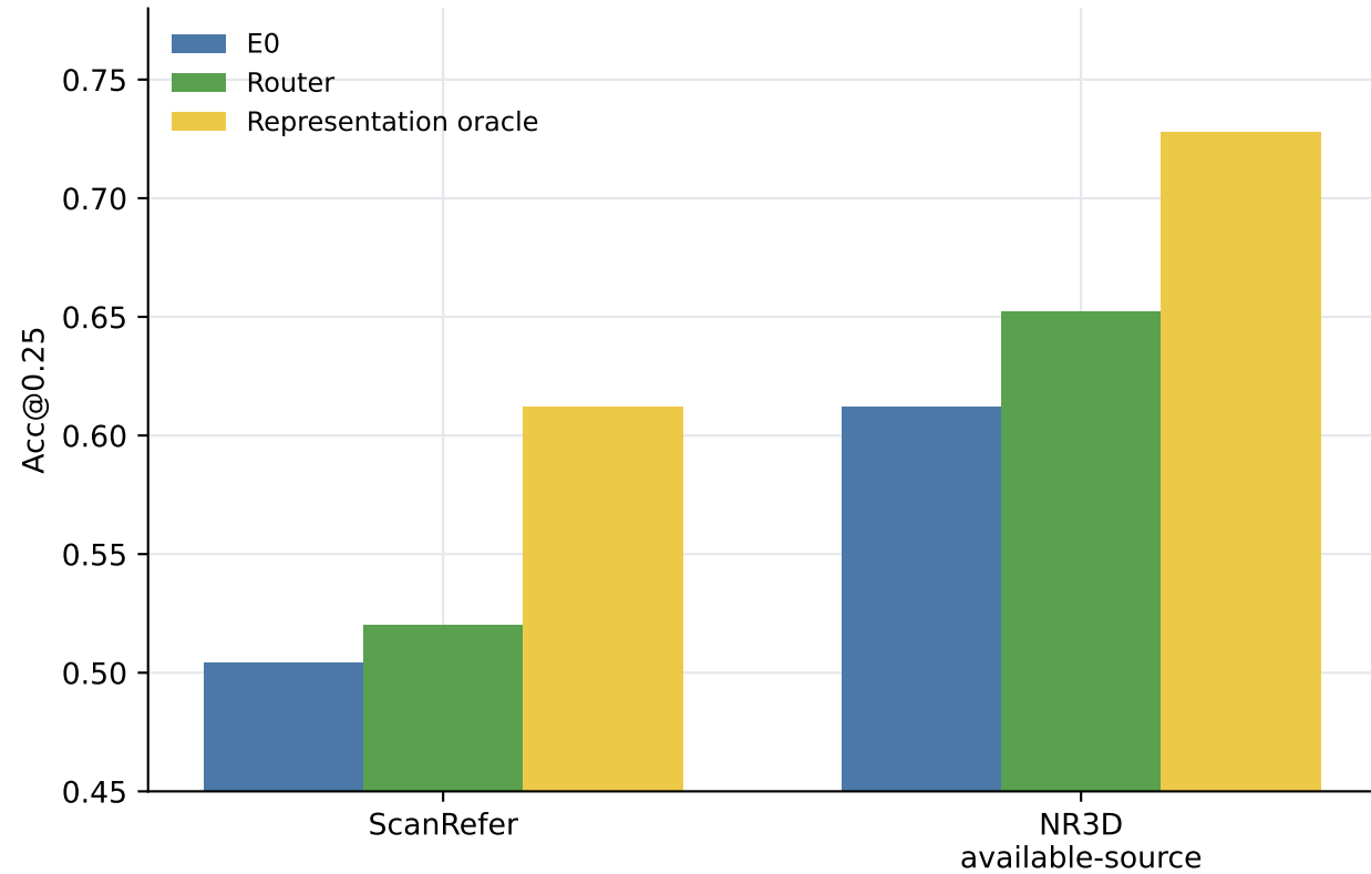
Representation Oracle Gap
