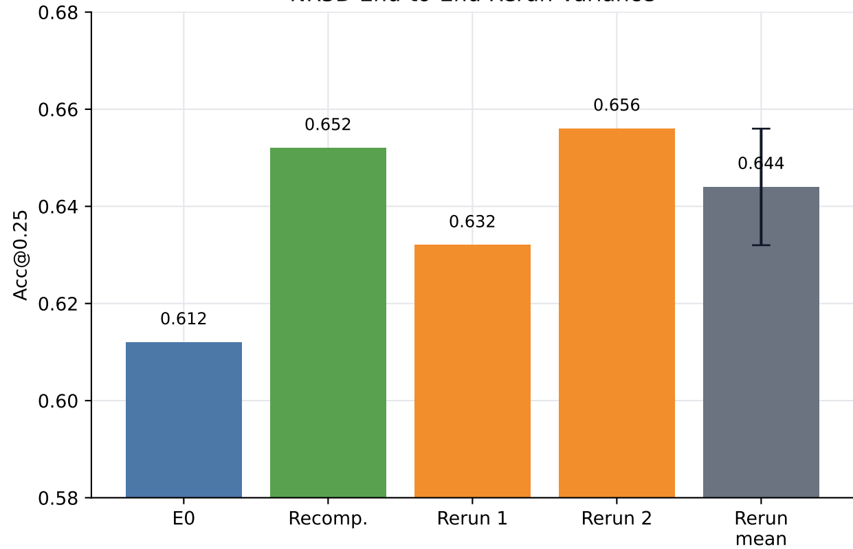
NR3D End-to-End Rerun Variance
