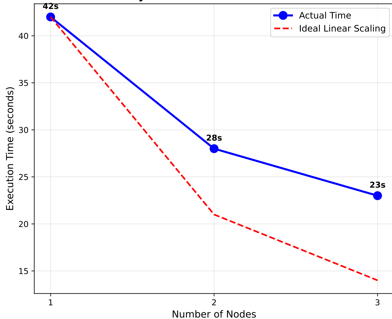
Scalability: Execution Time vs Cluster Size
