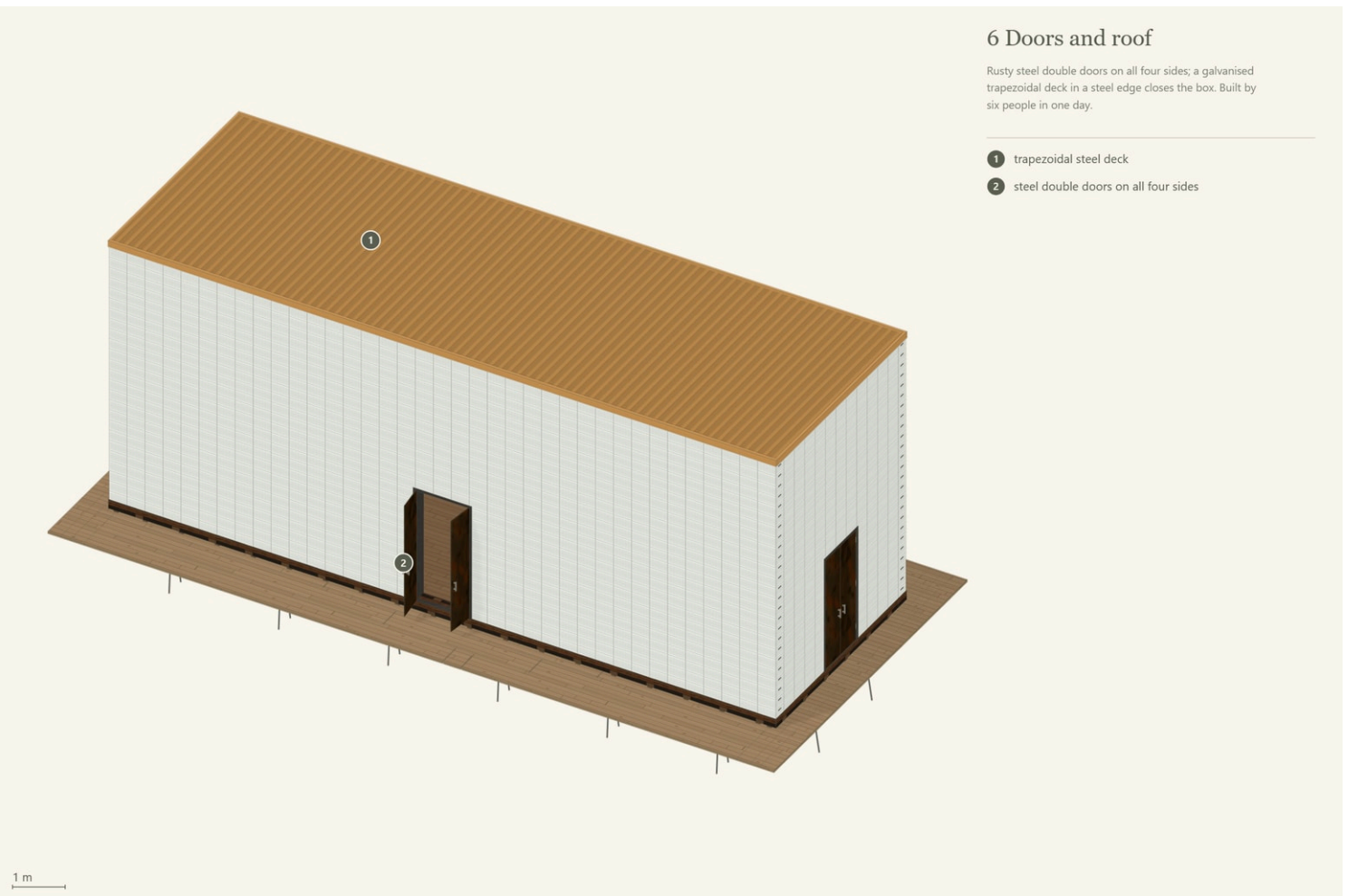
7 Step 6 Doors and roof
