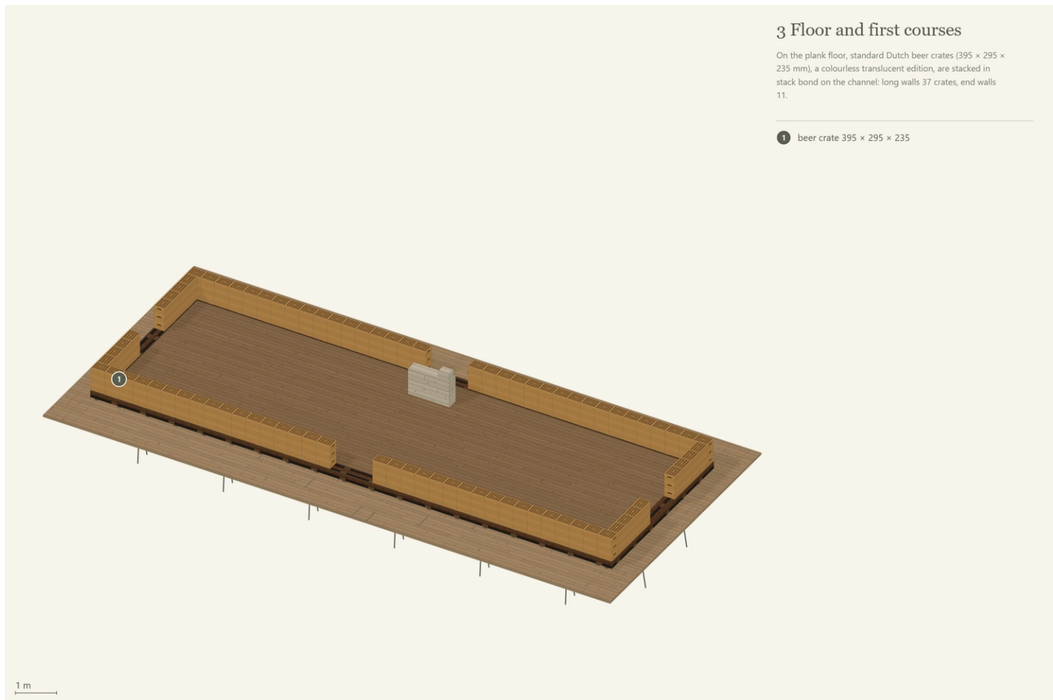
4 Step 3 Floor and first courses
