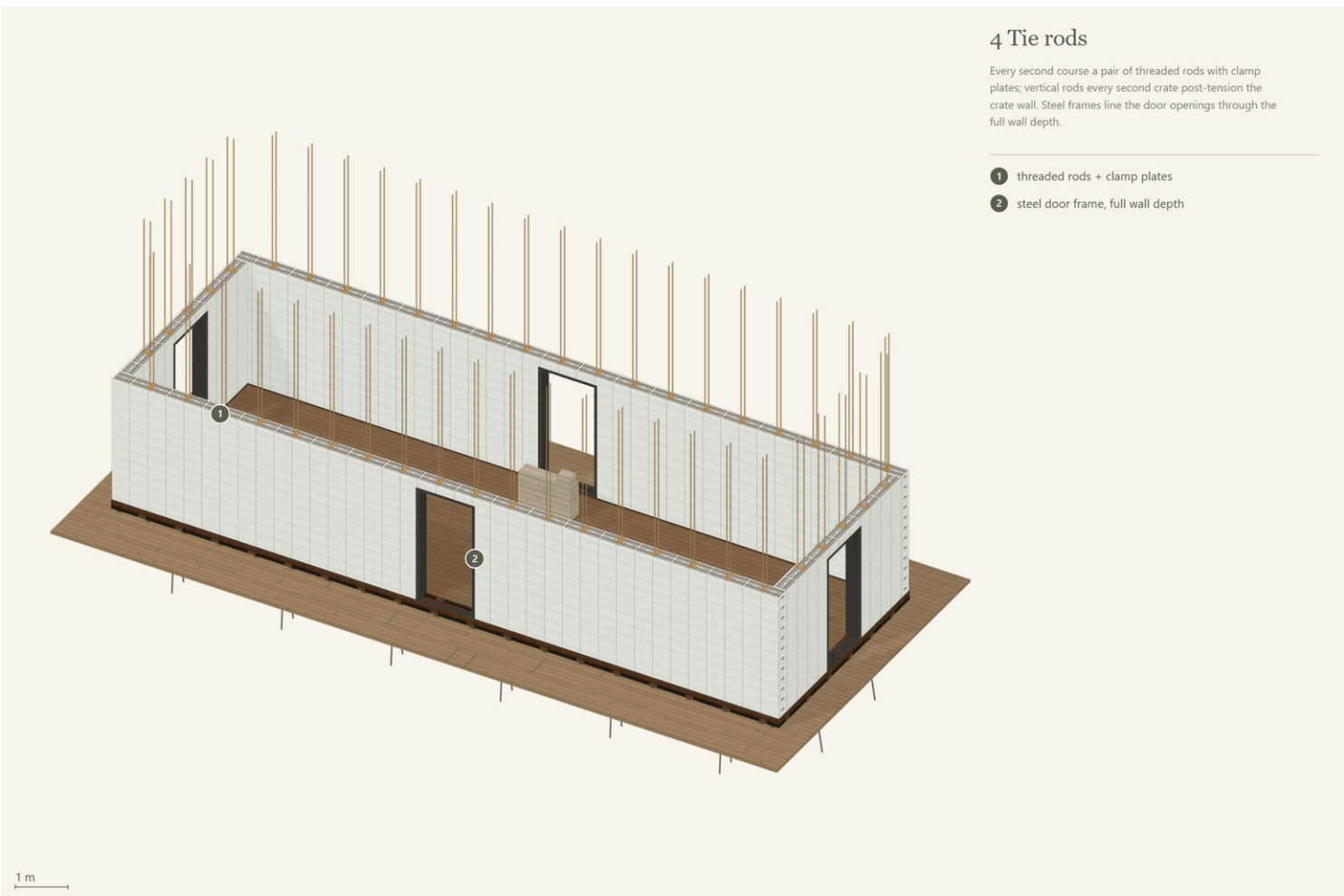
5 Step 4 Tie rods
