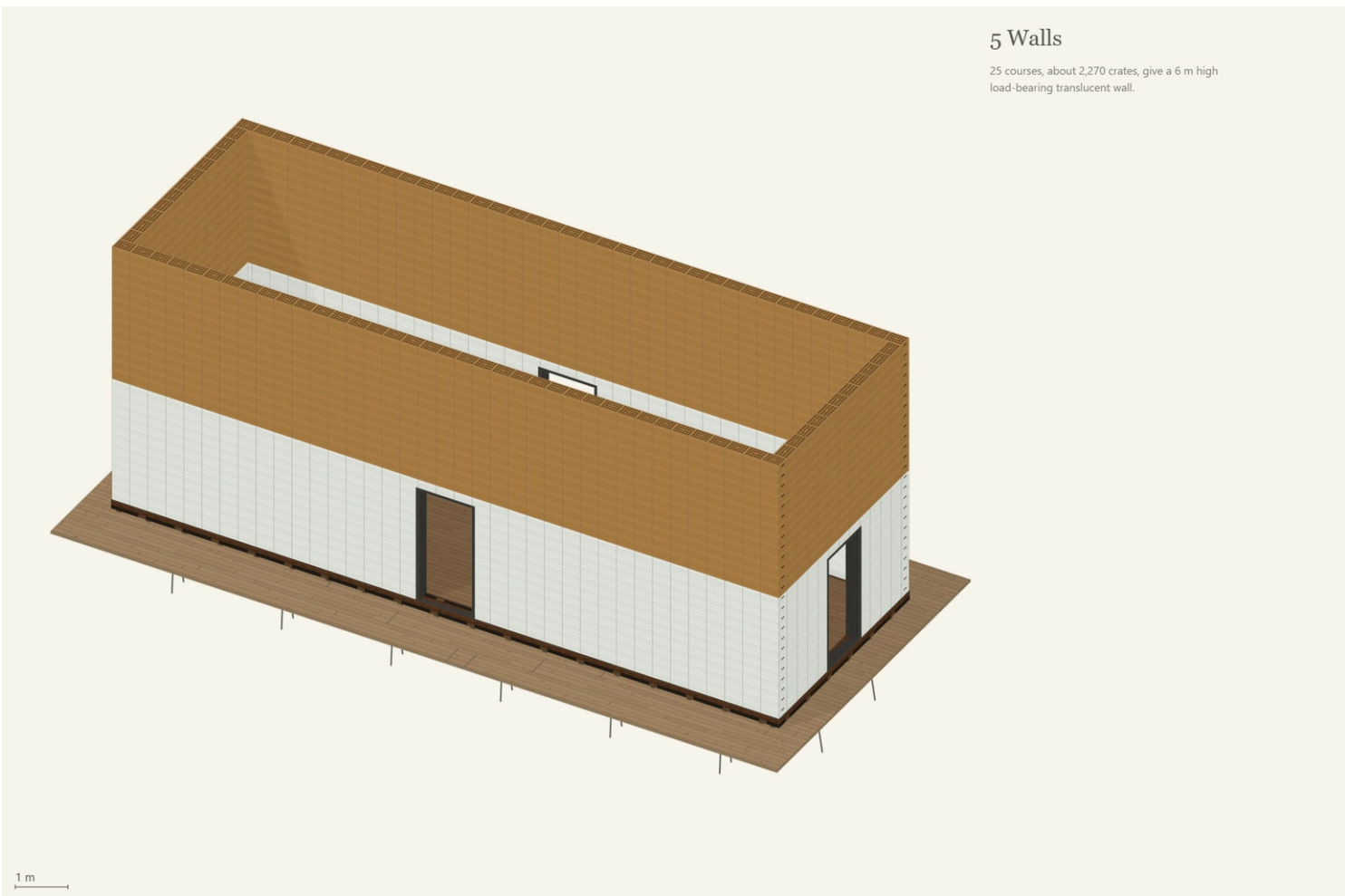
6 Step 5 Walls
