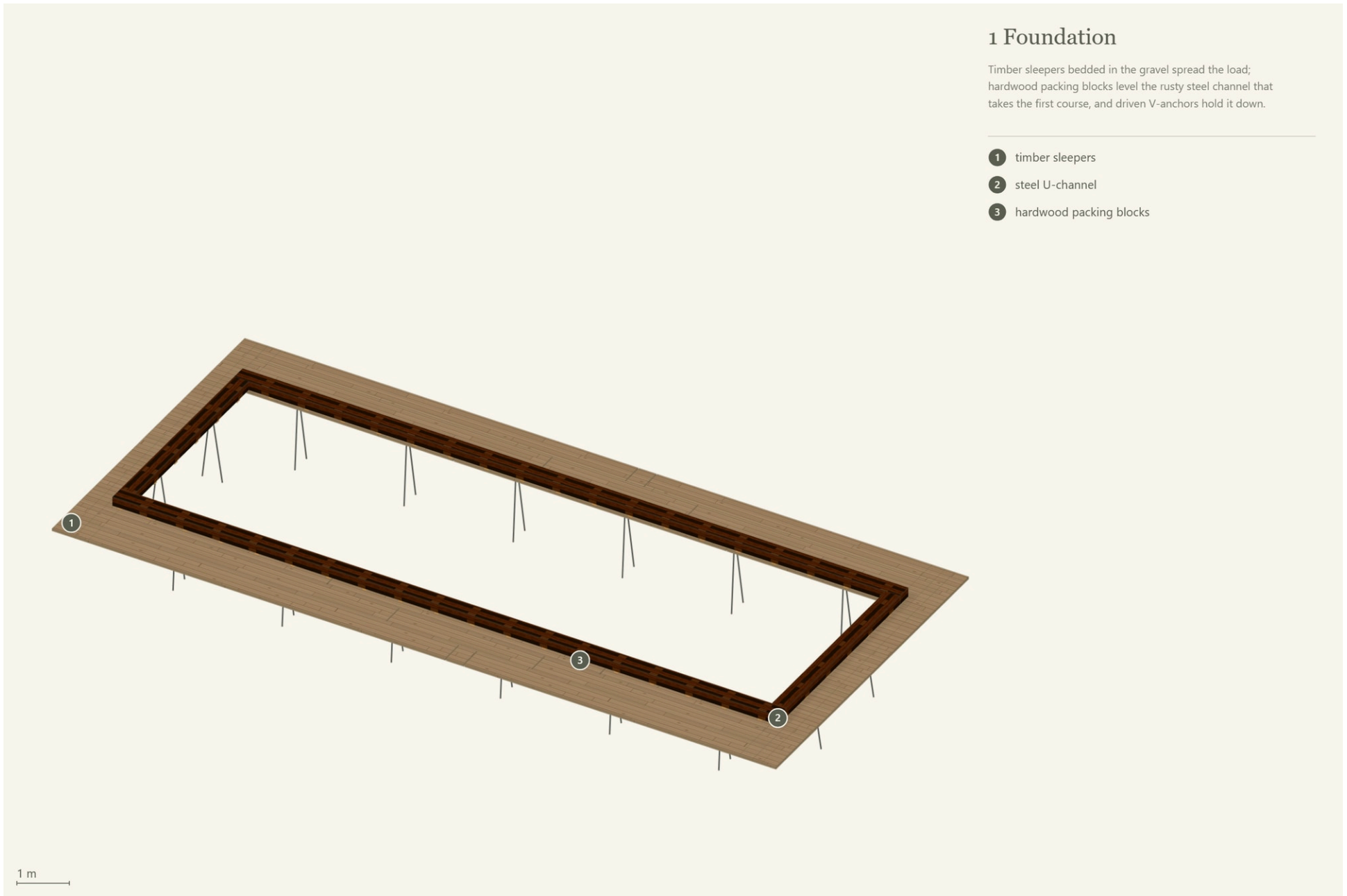
2 Step 1 Foundation
