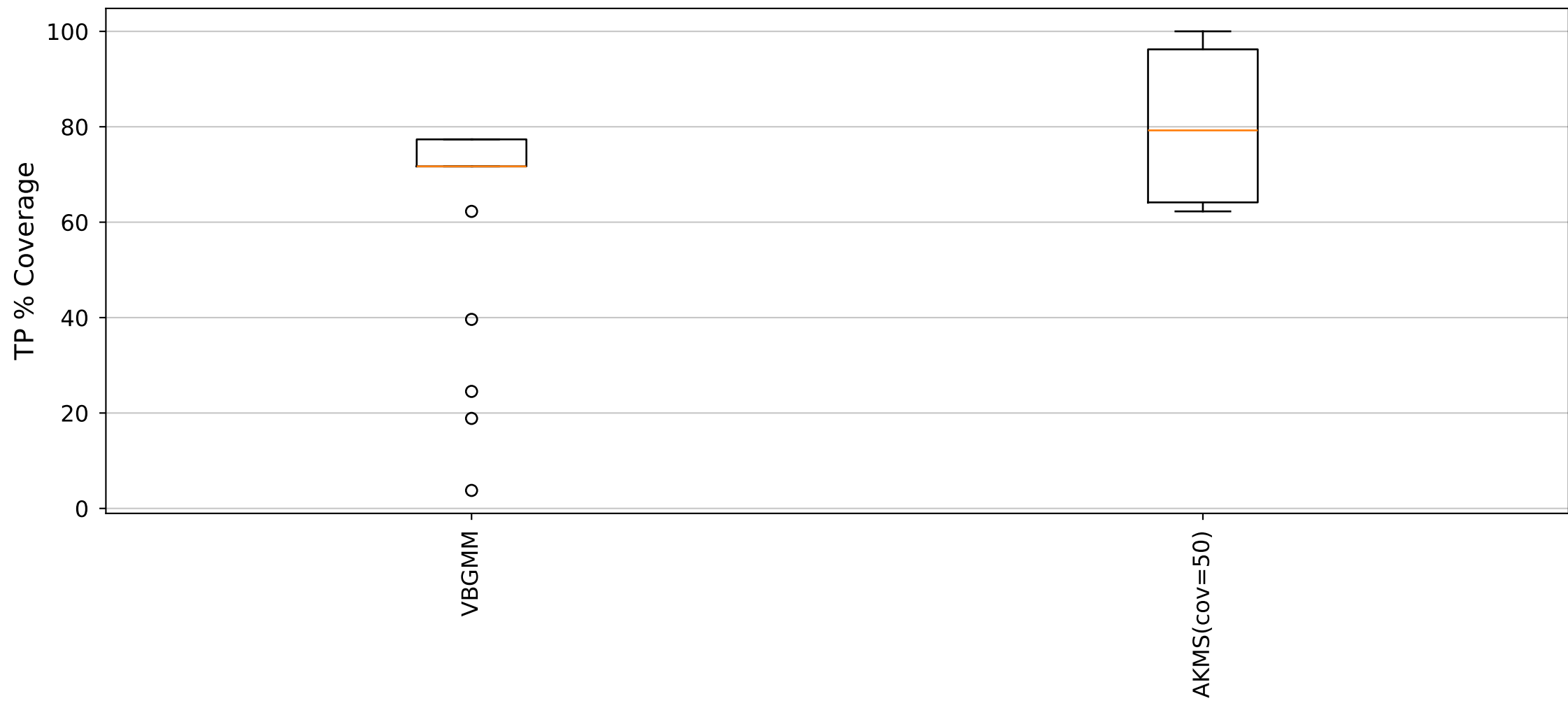
YARA Rules TP Distribution (Cluster3_Size53 dataset)
