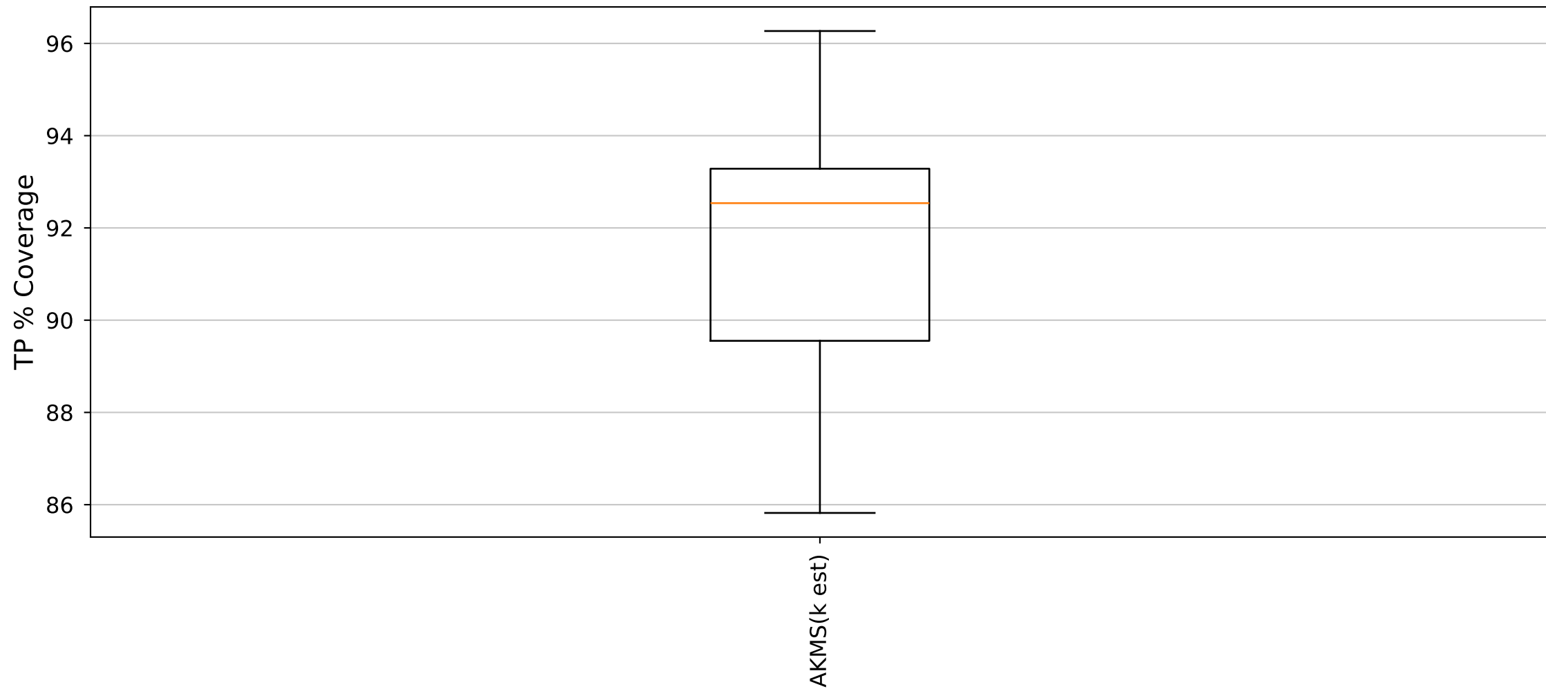
YARA Rules TP Distribution (Cluster0_Size134 dataset)
