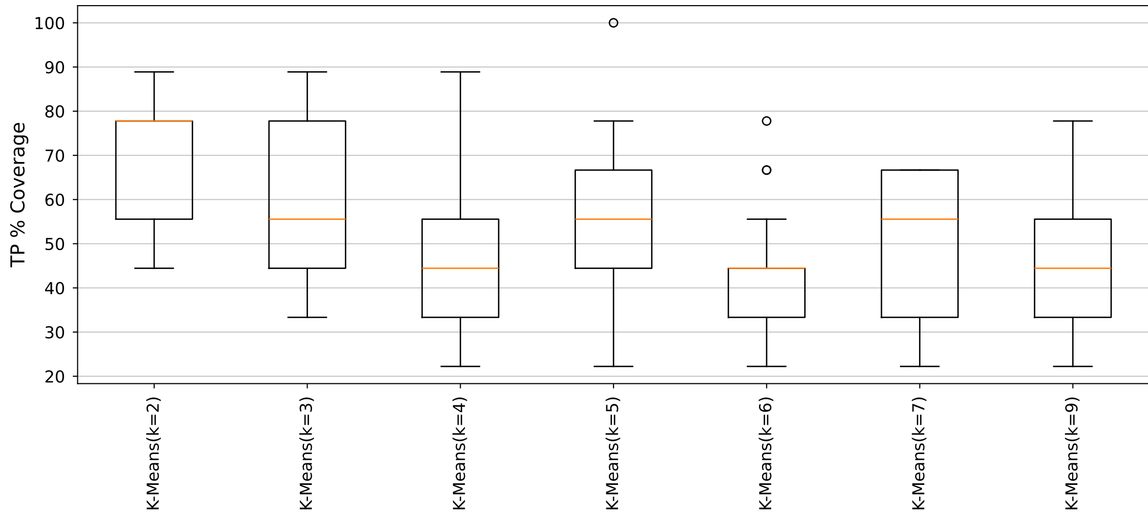
YARA Rules TP Distribution (Cluster11_Size9 dataset)
