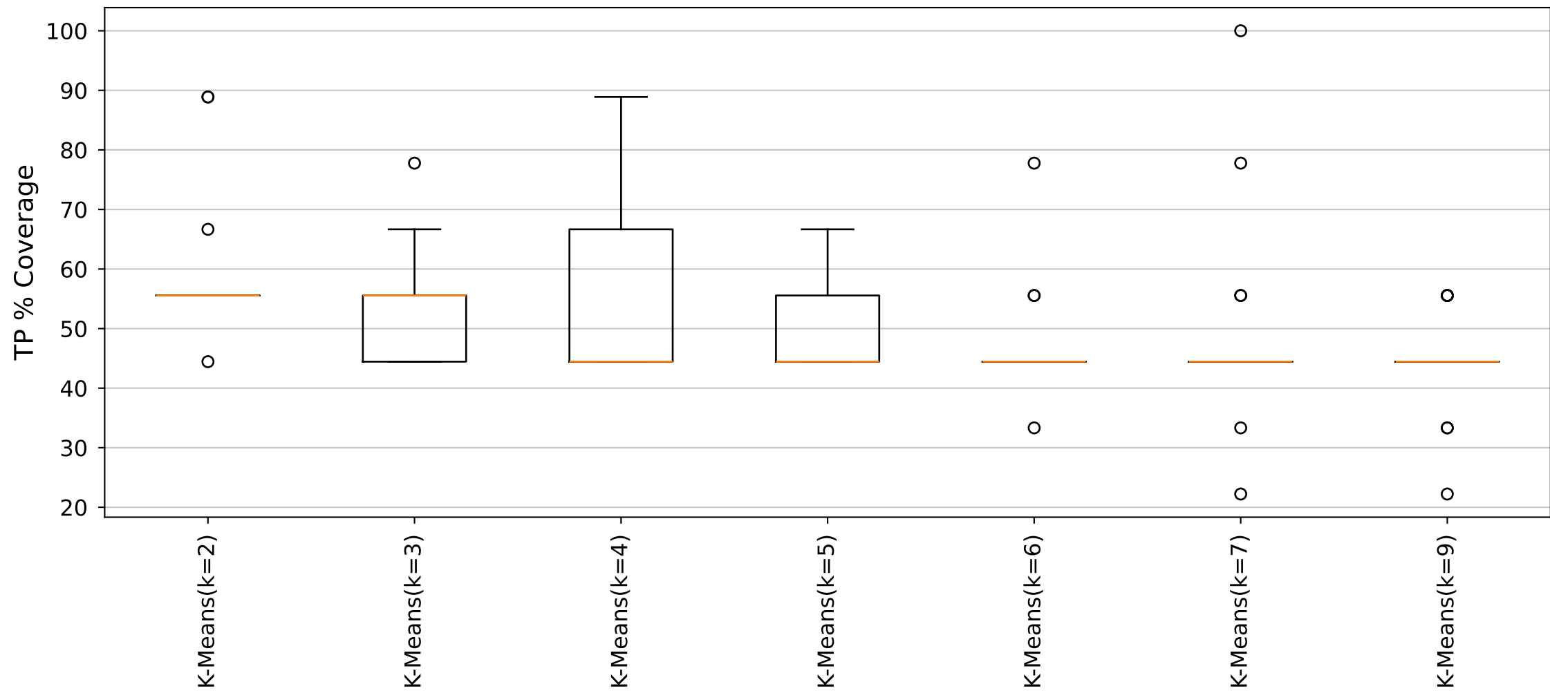
YARA Rules TP Distribution (Cluster12_Size9 dataset)
