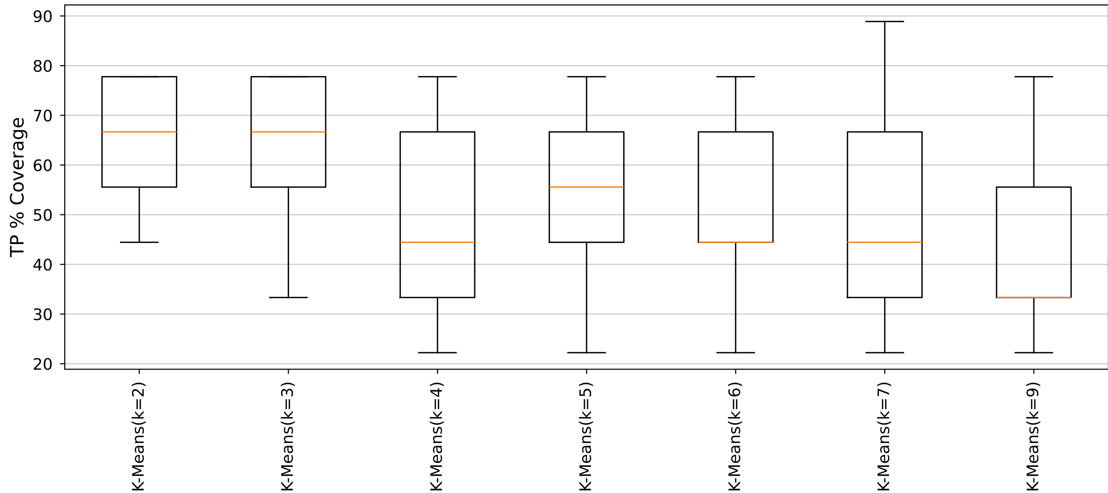
YARA Rules TP Distribution (Cluster14_Size9 dataset)
