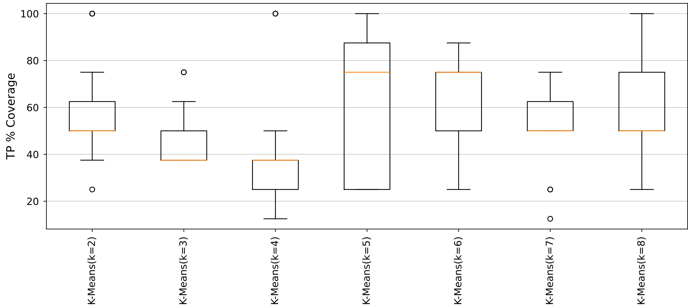
YARA Rules TP Distribution (Cluster16_Size8 dataset)
