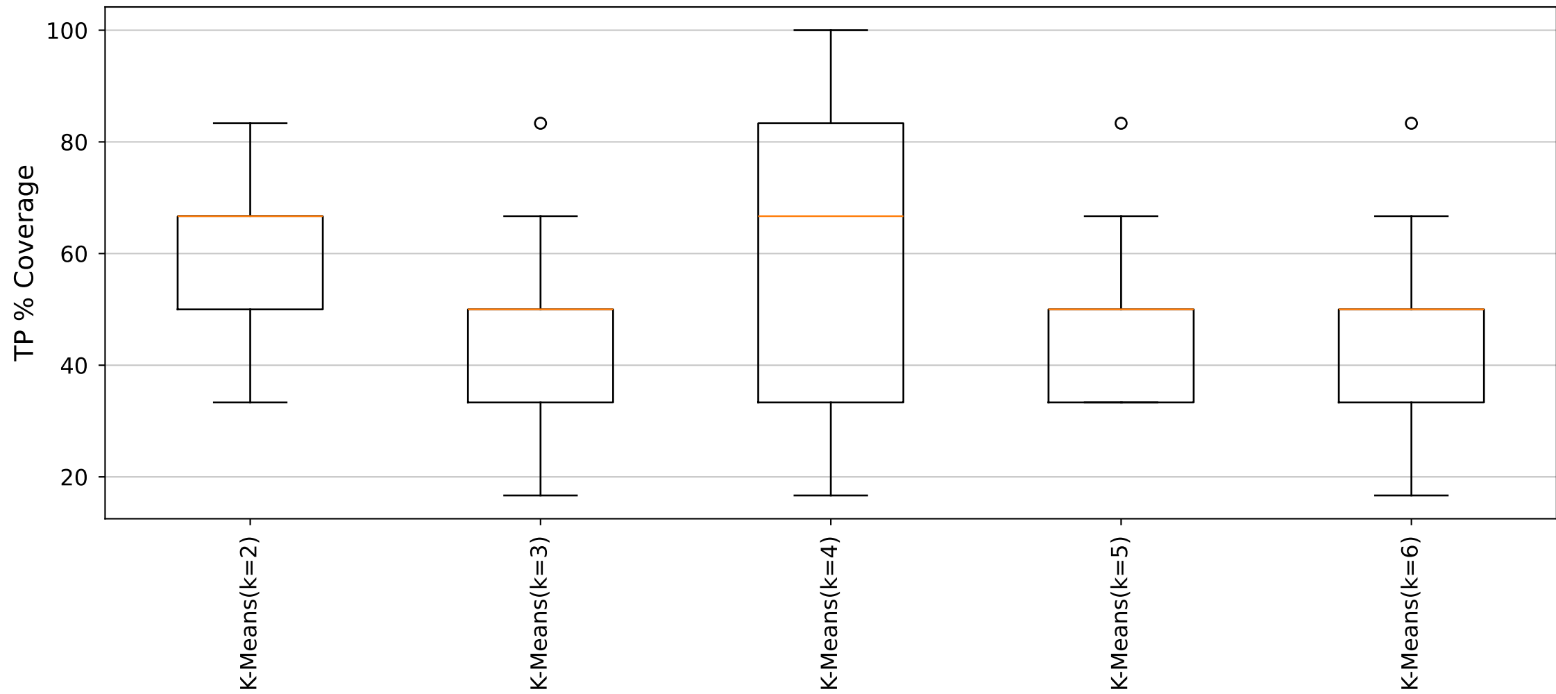
YARA Rules TP Distribution (Cluster18_Size6 dataset)
