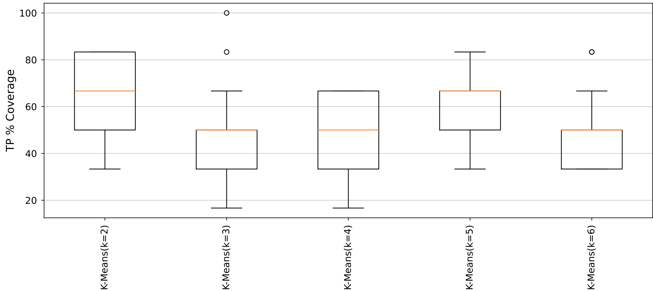
YARA Rules TP Distribution (Cluster19_Size6 dataset)
