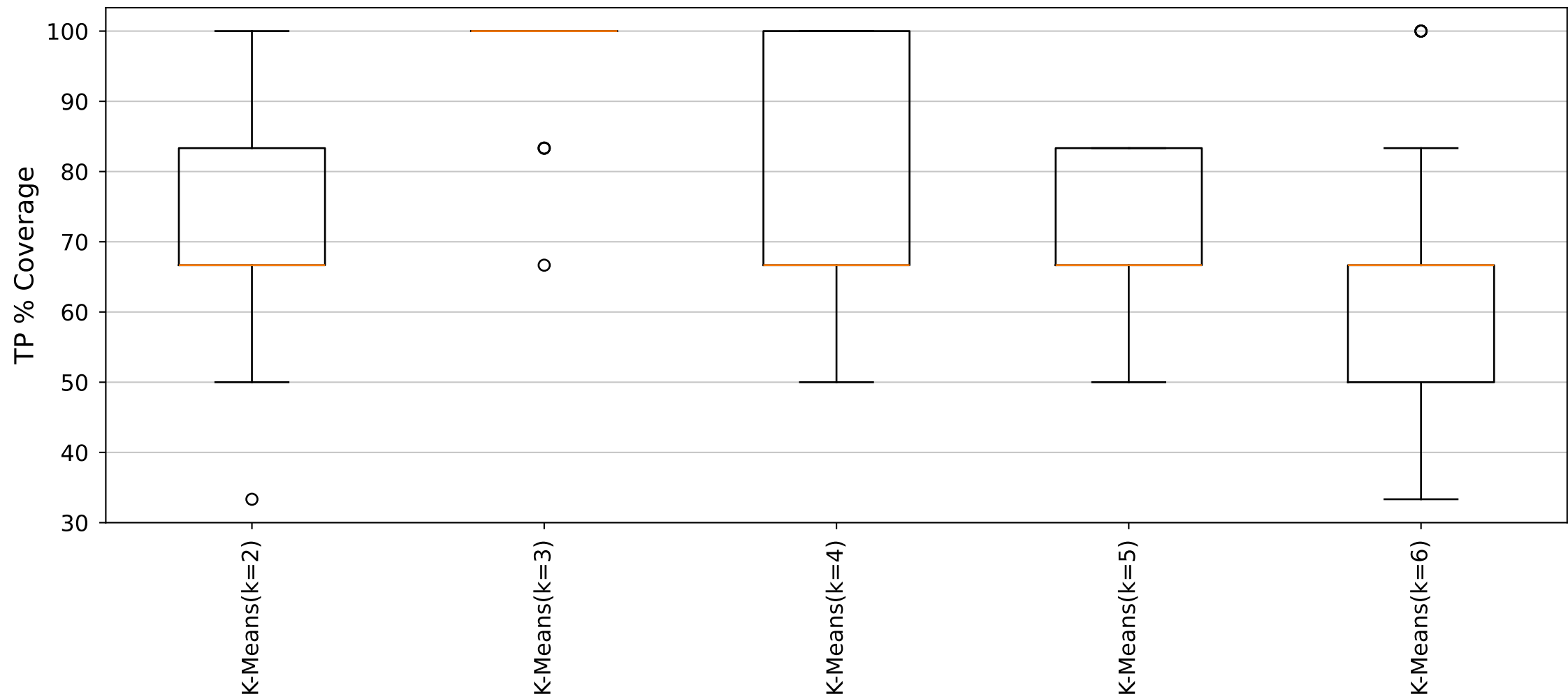
YARA Rules TP Distribution (Cluster23_Size6 dataset)
