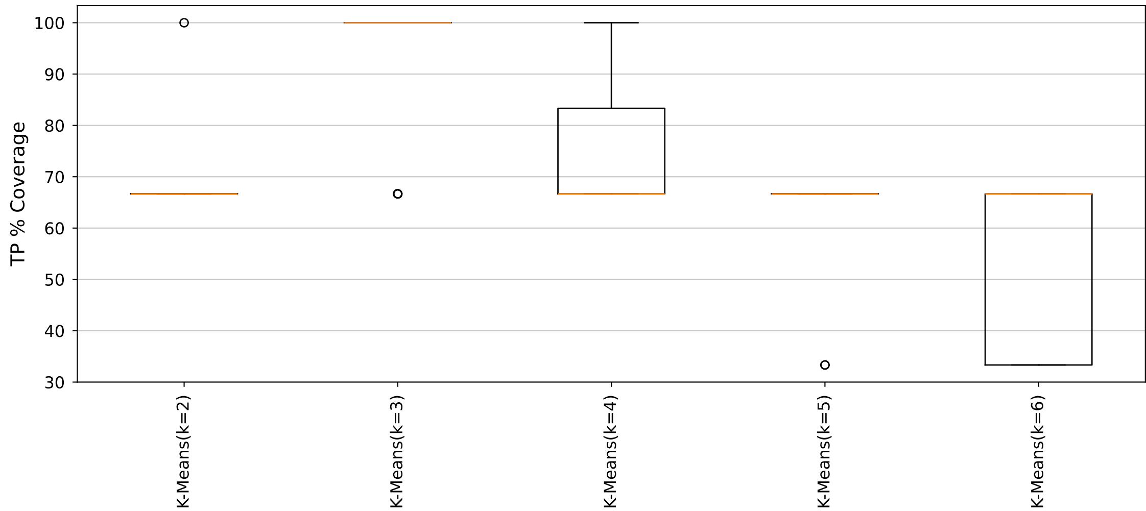
YARA Rules TP Distribution (Cluster26_Size6 dataset)
