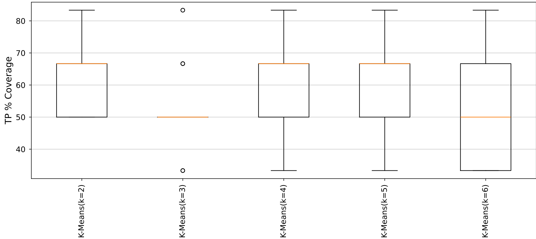
YARA Rules TP Distribution (Cluster27_Size6 dataset)
