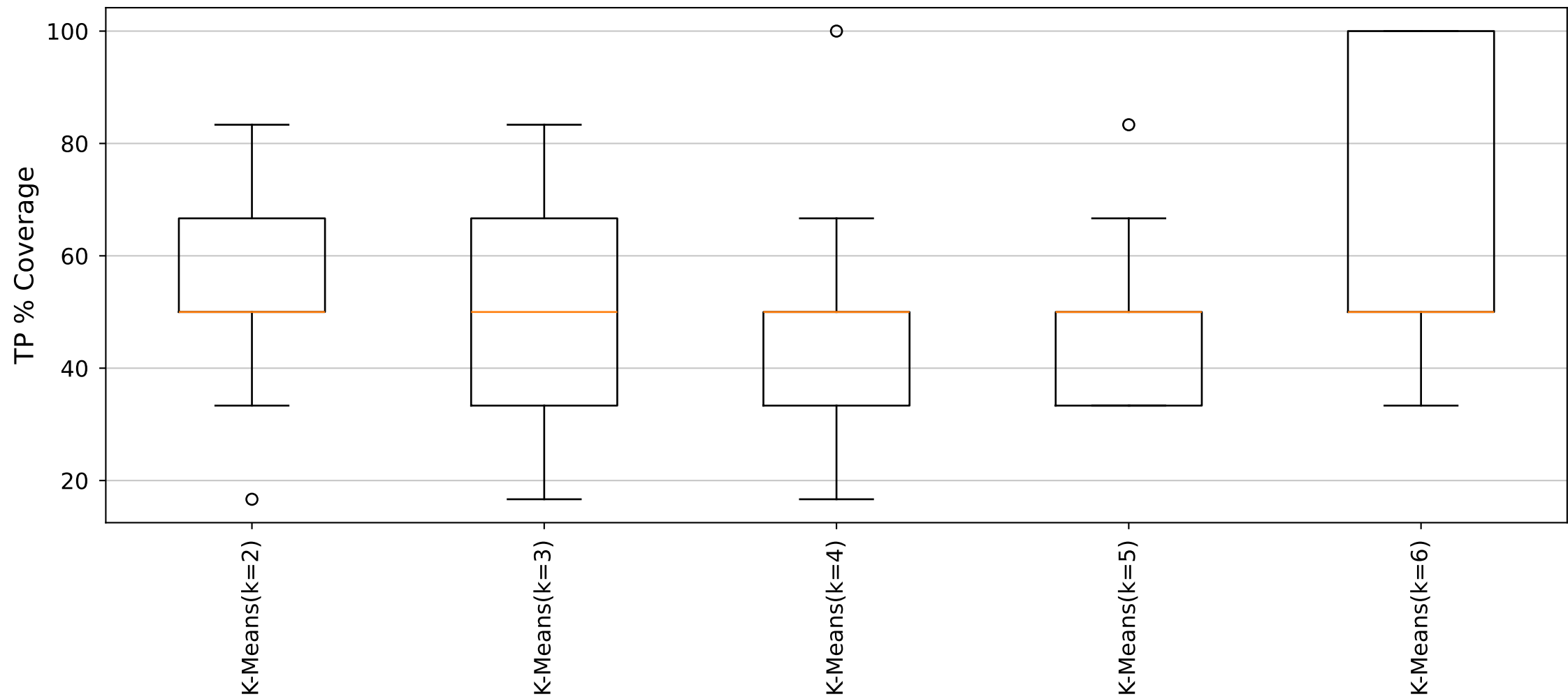
YARA Rules TP Distribution (Cluster29_Size6 dataset)
