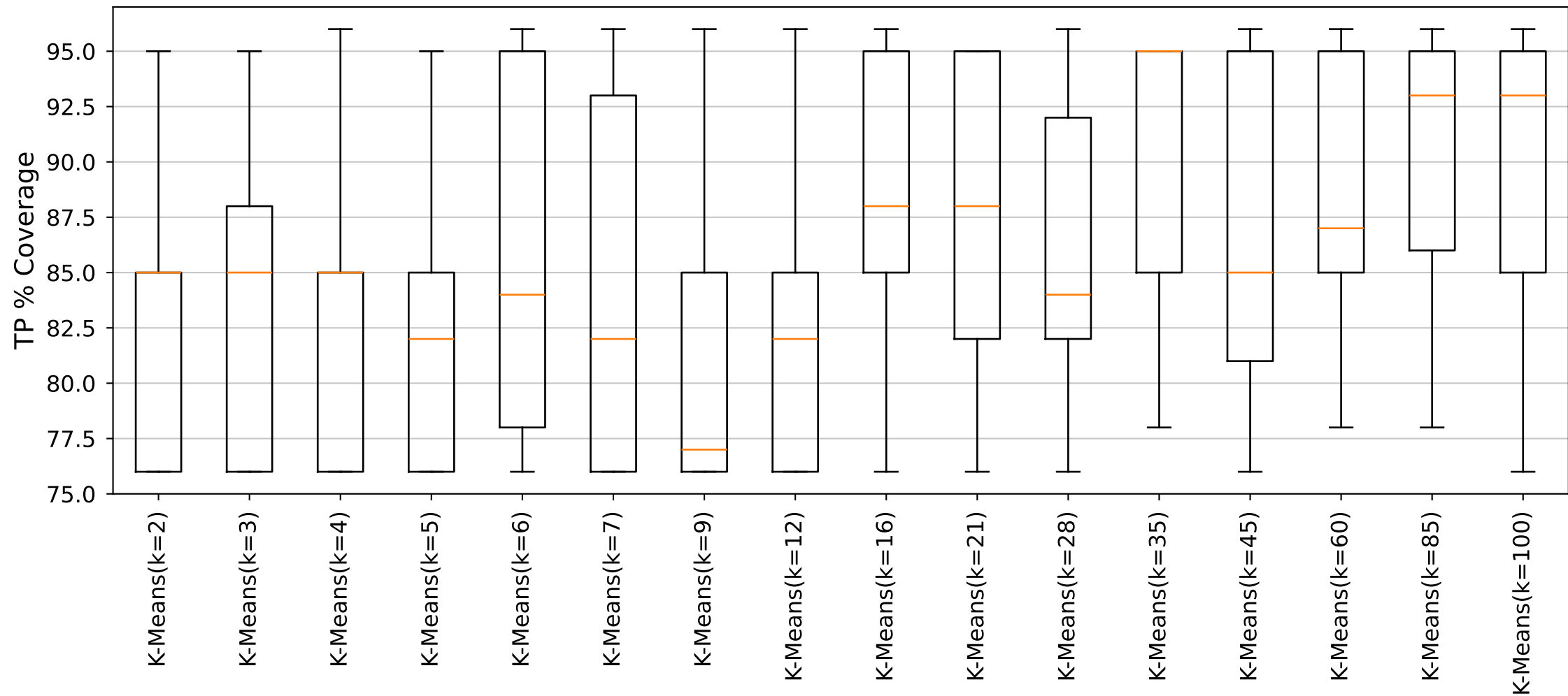
YARA Rules TP Distribution (Cluster2_Size100 dataset)
