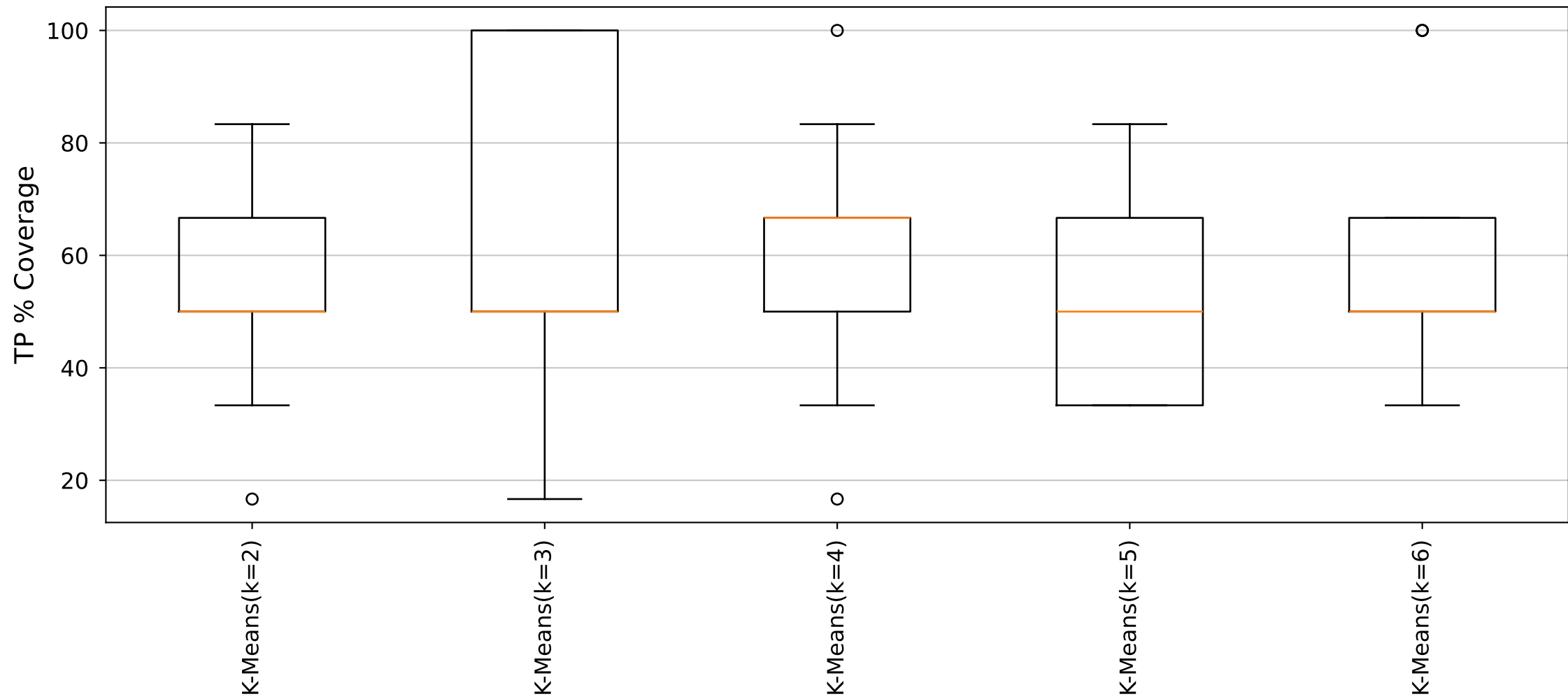
YARA Rules TP Distribution (Cluster31_Size6 dataset)
