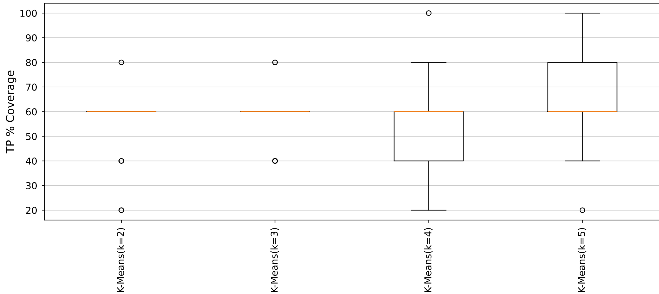
YARA Rules TP Distribution (Cluster36_Size5 dataset)
