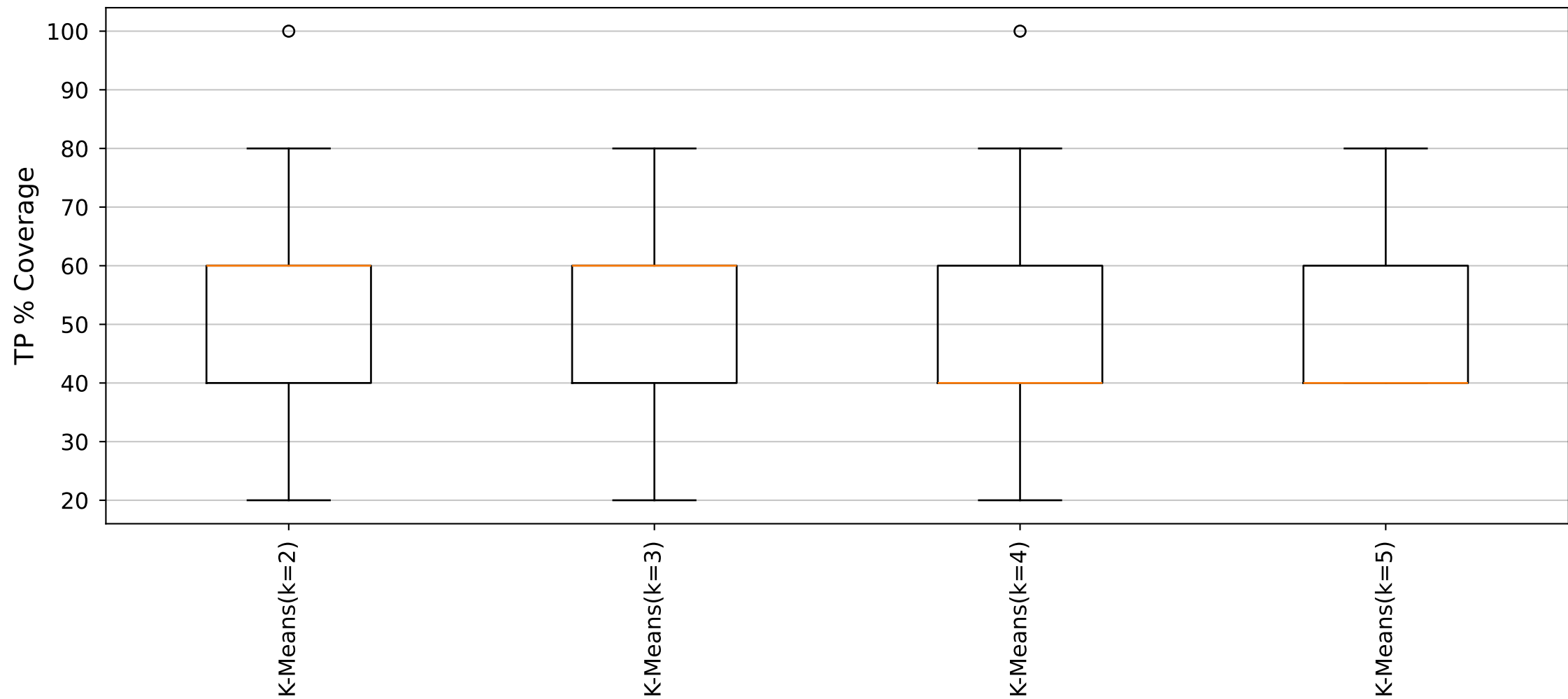
YARA Rules TP Distribution (Cluster37_Size5 dataset)
