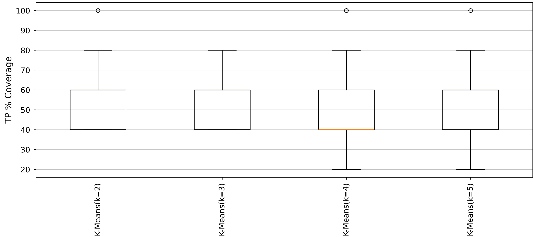
YARA Rules TP Distribution (Cluster38_Size5 dataset)
