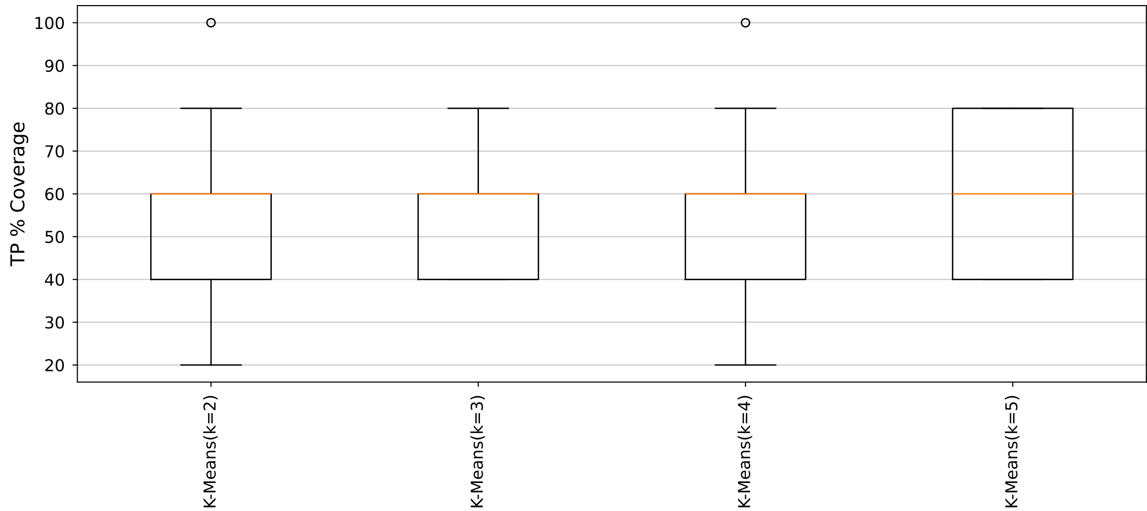
YARA Rules TP Distribution (Cluster39_Size5 dataset)
